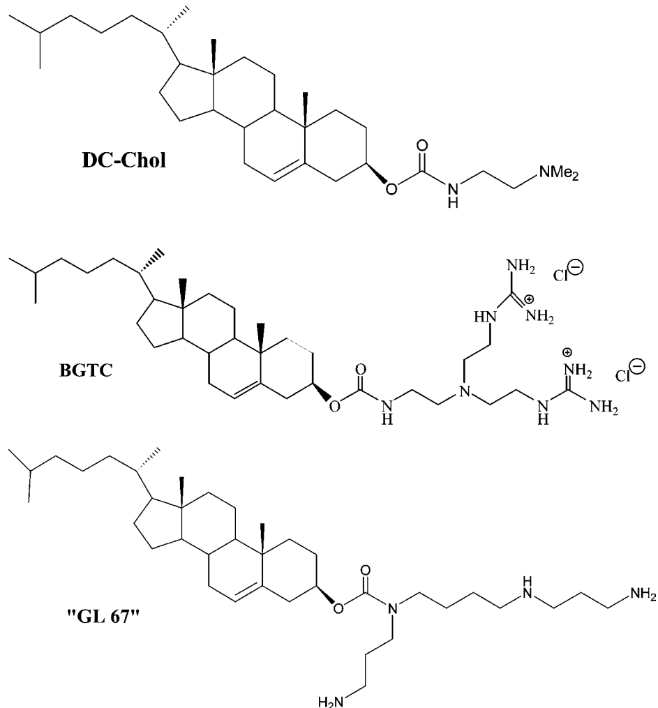
Scheme 1. Some Structures of Cationic Lipids with a Cholesteryl Lipidic Moiety
