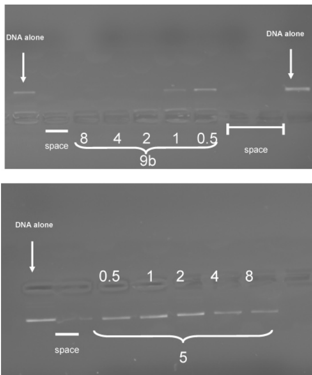
Figure 1. DNA binding ability of phosphoramidate 9b and cholesteryl 5 .
