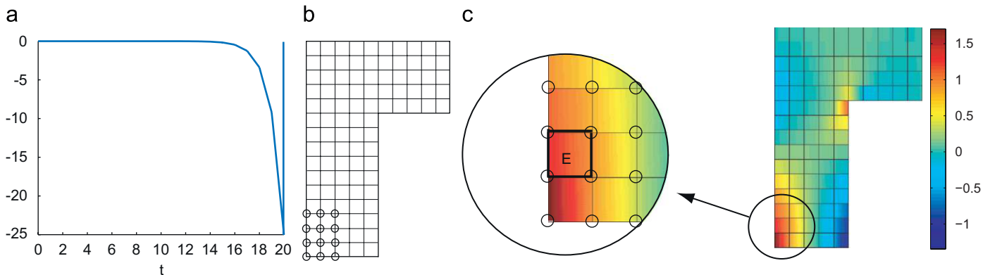
Fig. 19. Evolution of \bar{\sigma}_y with respect to time (a), nodes involved in the enrichment through the PUM (b), and definition of zone E (c).
