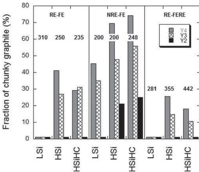
Fig. 5. Effect of silicon and carbon contents on chunky graphite amount. Numbers are nodule counts ( \text{mm}^{-2} ) measured at the bottom of Y2 blocks.
