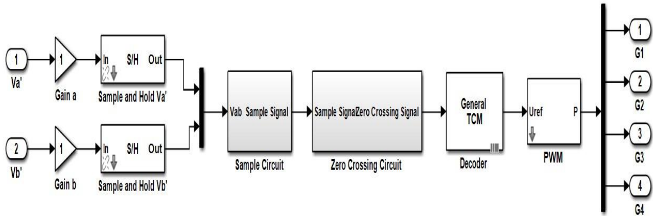
Fig. 5. Zero crossing Matlab Circuit.
