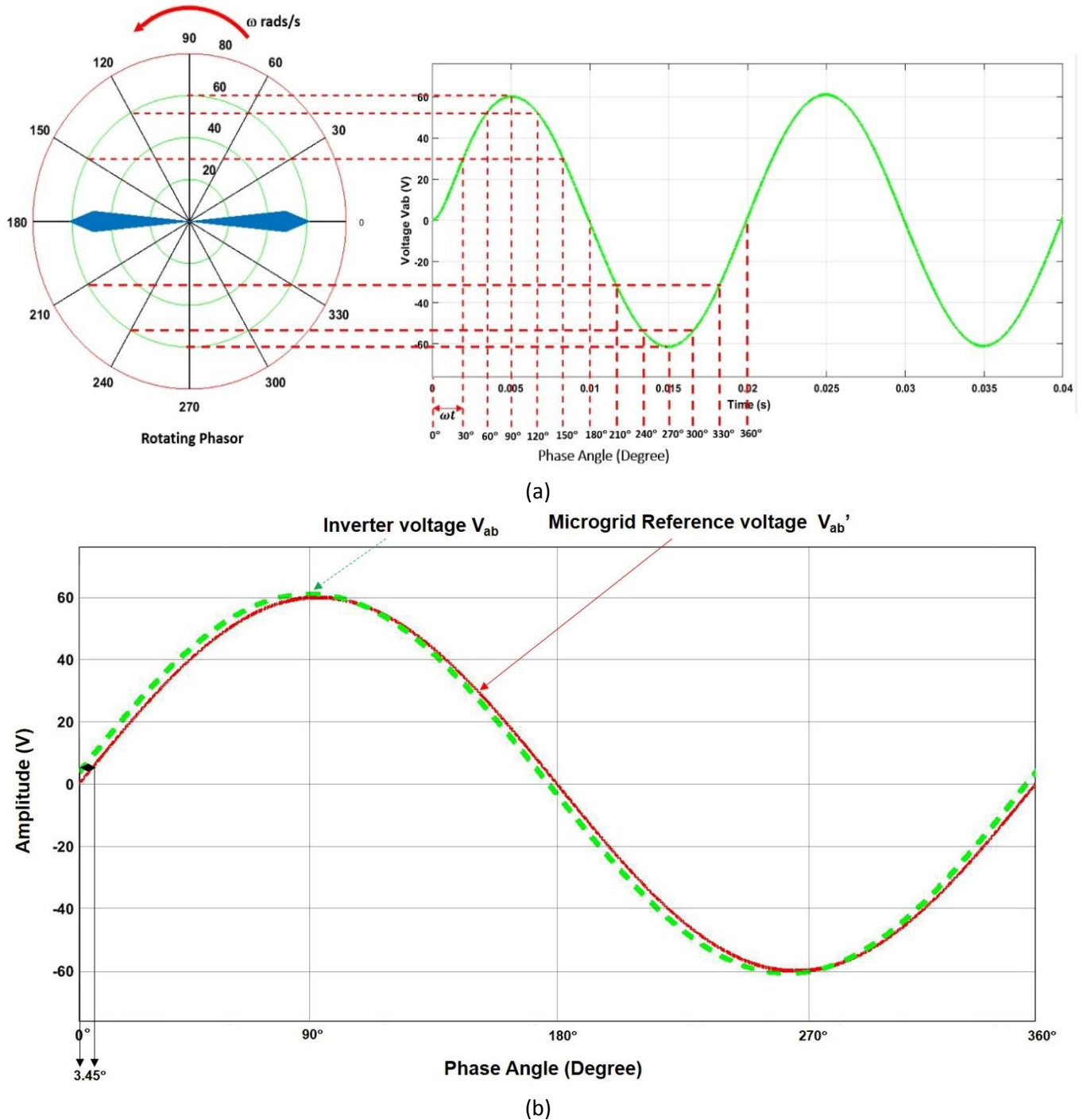
Fig. 11. Phase Synchronization for (a) microgrid output voltage and (b) inverter and microgrid reference voltage.
