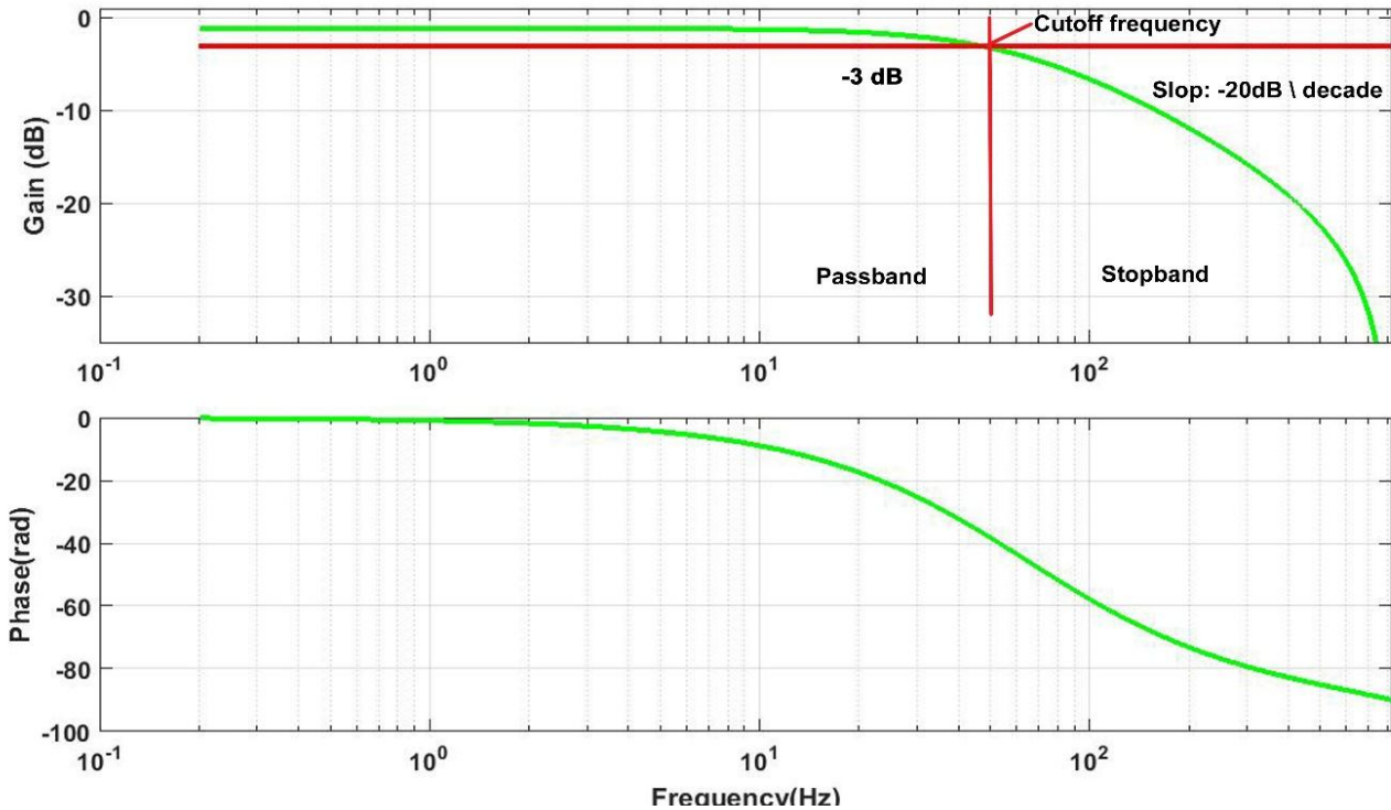
Fig. 7. The output lowpass LC filter gain-magnitude frequency response.
