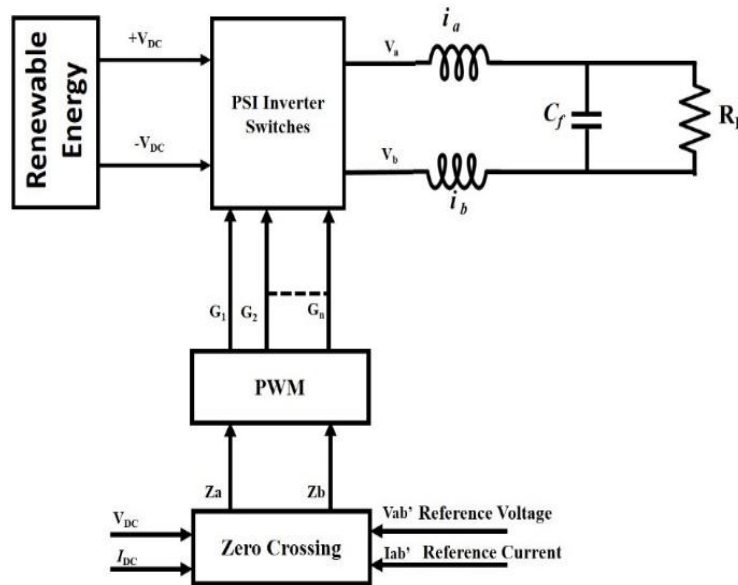
Fig. 1. Block diagram of PSI system.
