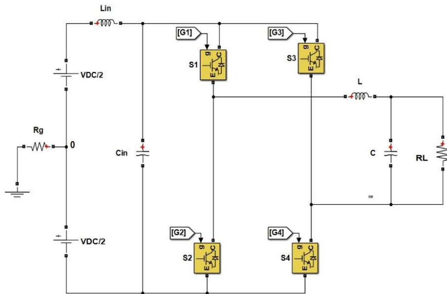
Fig. 2. Single phase half bridge inverter.
