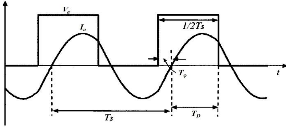
Fig. 4. Half phase PSI voltage and current.
