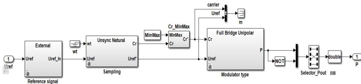
Fig. 3. Matlab circuit of the PWM controller.
