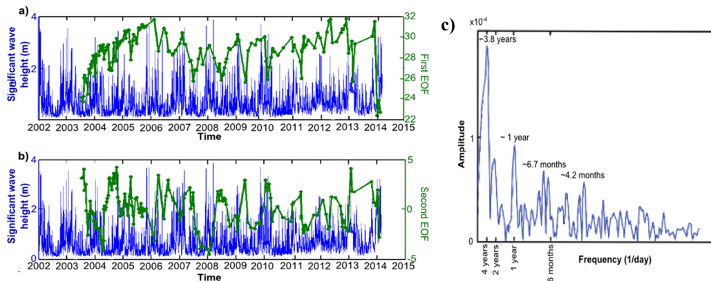
Figure 3: Empirical Orthogonal Functions (EOF) analyses from 2002 to 2014. (a) Correlation between significant wave height ( H_s ) and the (a) first EOF and (b) second EOF. (c) Spectral analysis of temporary amplitude.
