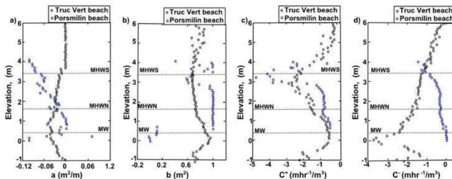
Figure 11: Optimal free parameters on the Truc Vert beach ( Castelle et al. 2014) and Porsmilin beach: (a) equilibrium slope a, (b) intercept the equilibrium wave energy b, (c) accretion coefficient C^+ , and (d) erosion coefficient C^- .
