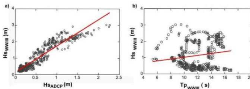
Figure 4: a) Scatter diagram of the significant wave height modelled WWIII ( H_{s_{wwIII}} ) and significant wave height ADCP ( H_{s_{ADCP}} ) and peaks period WWIII ( T_{p_{wwIII}} ), the solid red line is the regression linear giving y = 1.5920x + 0.1548 . b) Scatter diagram of the significant wave height model WWIII ( H_{s_{wwIII}} ) and peak period model WWIII ( T_{p_{wwIII}} ), the solid red line is the regression linear giving y = 0.5593x - 3.6545 .
