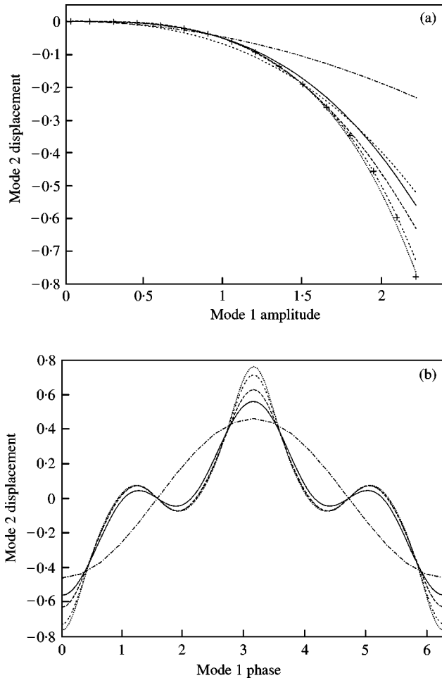
Figure 4. Convergence of the first NNM invariant manifold. In plot (a): —, asymptotic; -·-·-, (1, 2); - - - -, (2, 4); ---, (3, 8); ·····, (4, 10); - - - - -, (5, 12); +, exact. In plot (b): —, asymptotic; -·-·-, (1, 2); ---, (3, 8); ·····, (4, 10); - - - - -, (5, 12). The parenthetical notation refers to the number of basis functions, (N_a, N_\phi) , used in the expansion. Plots (a) and (b) illustrate cross-sections P_2(a, 0) , and P_2(2.22, \phi) respectively.
