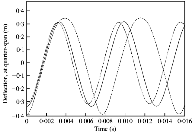
Figure 14. Time response for various second NNM solutions: —, Galerkin manifold; ---, asymptotic manifold; -·-·-, one mode solution; ····, exact. Again, the Galerkin manifold and exact solutions are indistinguishable.
