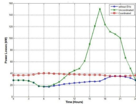
Fig. 42. Power losses of Feeder Fdr2
