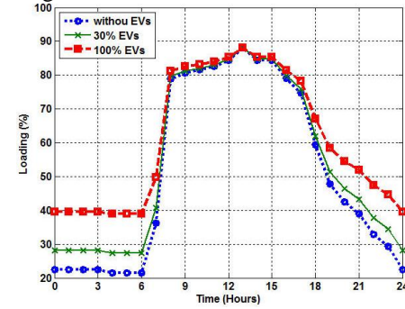
Fig. 20. Load profile of transformer TP4
