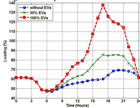
Fig. 25. Load profile of transformer TP1
