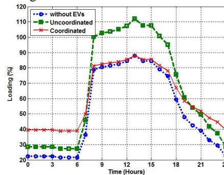
Fig. 38. Load profile of transformer TP4
