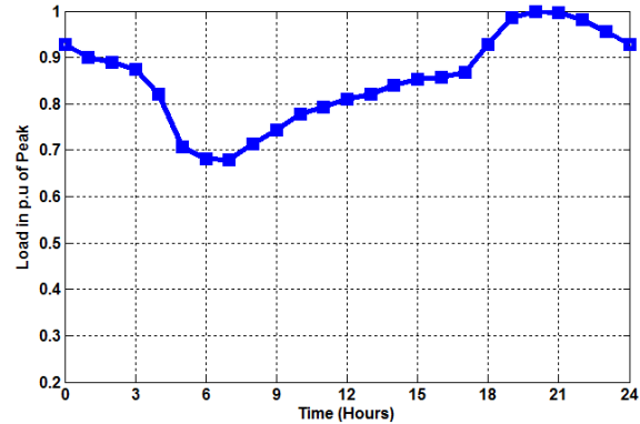
Fig. 7. Egyptian daily load curve [13]
