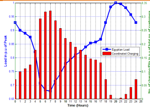
Fig. 4. Coordinated charging corresponding to Egyptian load type
