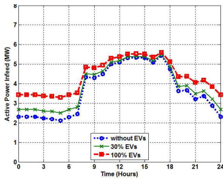
Fig. 17. Load profile of Feeder Fdr1
