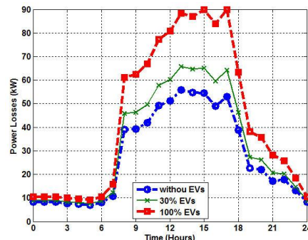
Fig. 12. Power losses of Feeder Fdr1
