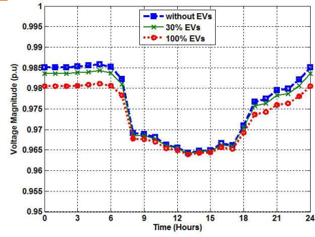
Fig. 22. Voltage profile at LP4
