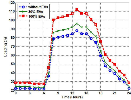
Fig. 14. Load profile of transformer TP4
