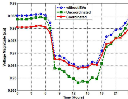
Fig. 40. Voltage profile at LP4
