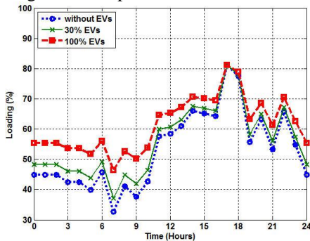
Fig. 19. Load profile of transformer TP1
