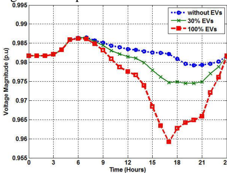
Fig. 27. Voltage profile at LP17
