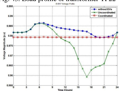
Fig. 45. Voltage profile at LP17
