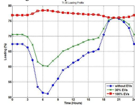
Fig. 31. Load profile of transformer TP30
