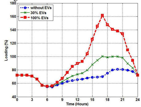
Fig. 26. Load profile of transformer TP2
