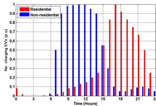
Fig. 1. Uncoordinated charging
