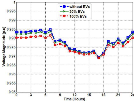
Fig. 21. Voltage profile at LP1
