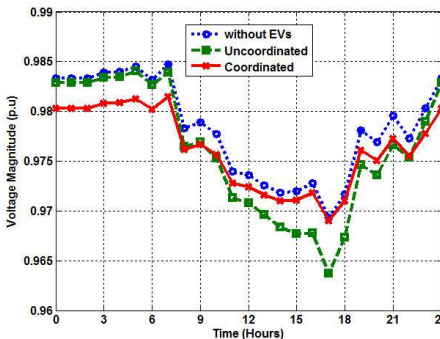
Fig. 39. Voltage profile at LP1
