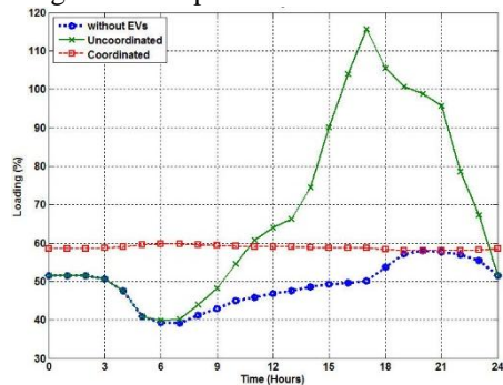
Fig. 43. Load profile of transformer TP22
