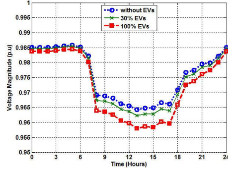
Fig. 16. Voltage profile at LP4
