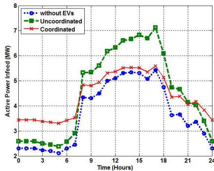
Fig. 35. Load profile of Feeder Fdr1
