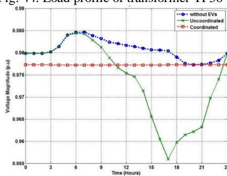
Figure 45: Voltage profile at LP32
