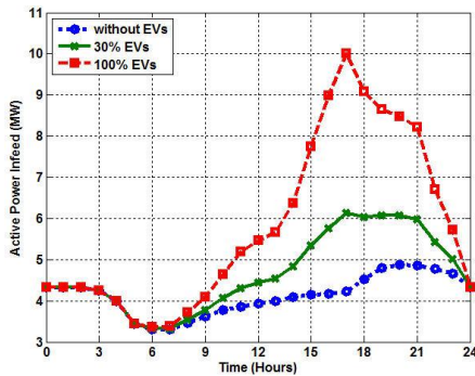
Fig. 23. Load profile of Feeder Fdr1
