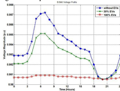
Fig. 34. Voltage profile at LP45
