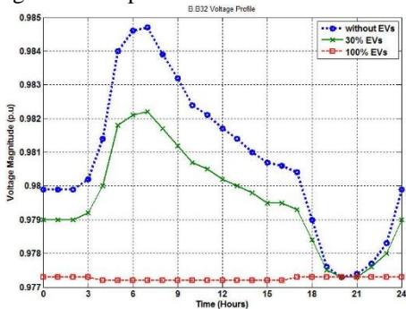
Fig. 33. Voltage profile at LP32
