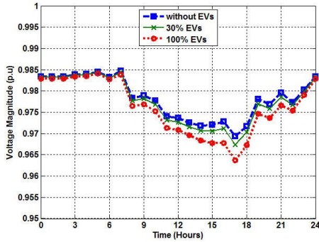
Fig. 15. Voltage profile at LP1
