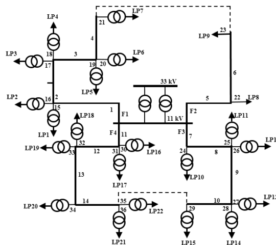
Fig. 9. RBTS Bus 2 Distribution Test System [15]
