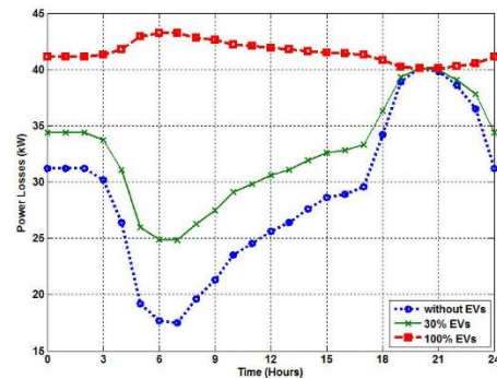
Fig. 30. Power losses of Feeder Fdr1
