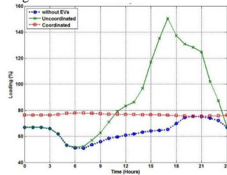
Fig. 44. Load profile of transformer TP36
