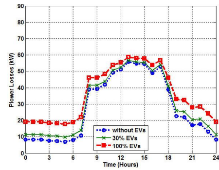
Fig. 18. Power losses of Feeder Fdr1
