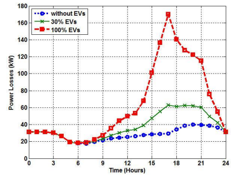
Fig. 24. Power losses of Feeder Fdr1
