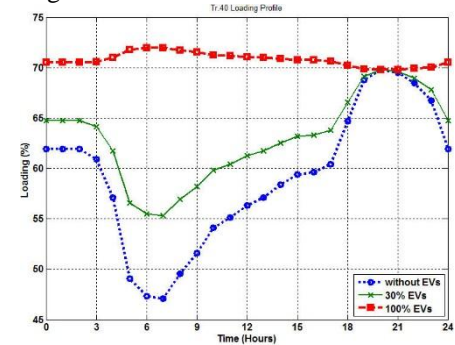
Fig. 32. Load profile of transformer TP40
