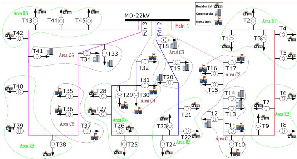
Fig. 10. ShC-D8 Distribution Test System
