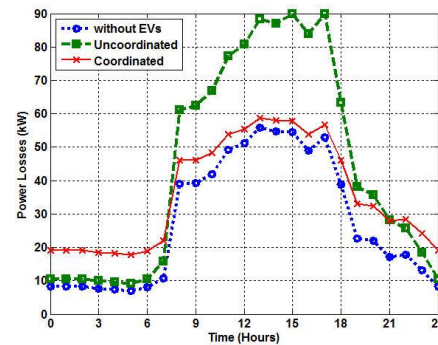
Fig. 36. Power losses of Feeder Fdr1
