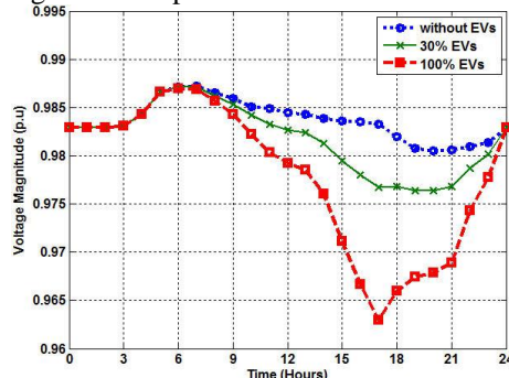
Fig. 28. Voltage profile at LP45
