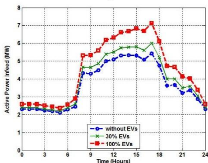
Fig. 11. Load profile of Feeder Fdr1
