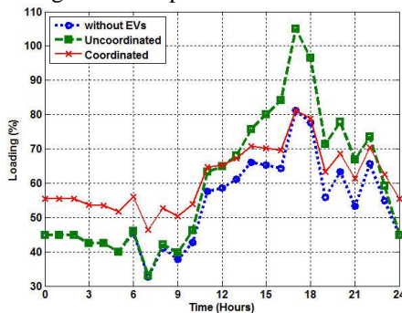
Fig. 37. Load profile of transformer TP1
