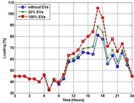
Fig. 13. Load profile of transformer TP1
