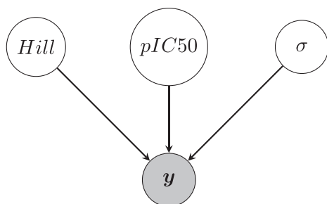
Figure 2. Statistical model for the generation of dose-response data. All non-shaded variables are parameters for which we wish to infer probability distributions. \mathbf{y} = \{y^{(1)}, \dots, y^{(K)}\} is the vector of all experimentally-recorded response data points.
