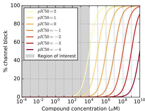
Figure 3. Large IC_{50} values are indistinguishable when they are orders of magnitude above the relevant concentration range. Here we show the effect of decreasing pIC_{50} (increasing IC_{50} ), while maintaining Hill = 1 . The shaded "region of interest" covers the minimum and maximum concentrations in the data published by Crumb et al. . As pIC_{50} decreases, there is no significant change to the dose-response curve across the relevant range of concentrations — all predictions are close to zero response. As a result we somewhat artificially 'cap' pIC_{50} priors to exclude pIC_{50} < -1 , otherwise (for datasets with no response signal) convergence of minimisation and MCMC algorithms is difficult if not impossible.
