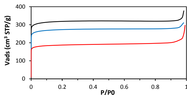
Figure 3: Nitrogen adsorption isotherms of as-made HKUST-1 powder (black/top), and HKUST-1 tablets pressed at 62MPa with as-made powder (blue/middle) or with powder fully activated prior compression (red/bottom).
