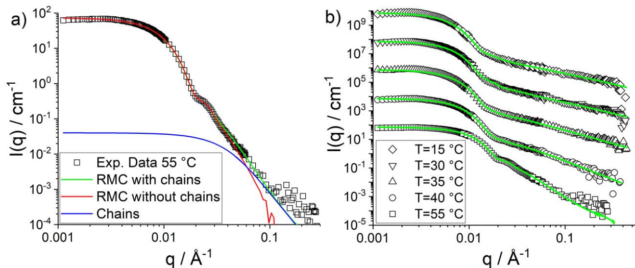
Figure 5: (a) Fitted chain and profile contributions to scattered intensity of a microgel (CC = 10 mol%) at 55^\circ\text{C} . (b) Temperature series from 15 to 55^\circ\text{C} of experimental intensities of the same microgel (symbols), compared to the model fits (solid lines).
