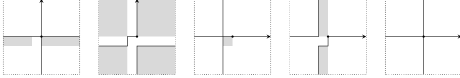
Figure 14: Dihomotopies on the flat torus.
