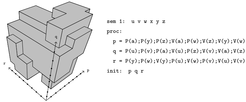
Figure 12: The geometric model of the Lipski algorithm.
