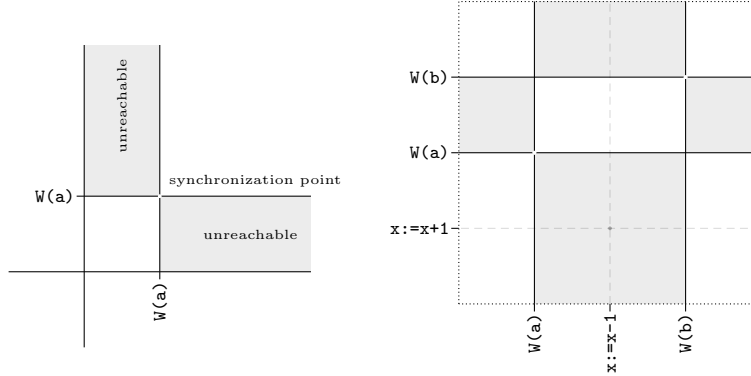
Figure 9: Binary synchronization: producer vs consumer on a flat torus (the opposite edges of the dotted frame are identified).
