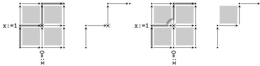
Figure 13: Comparing the discrete and the continuous approaches: an admissible directed path that meets a forbidden point and a possible replacement for it.
