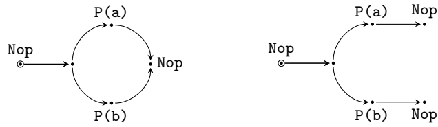
Figure 4: Conservative process may be obtained by duplicating a vertex.
