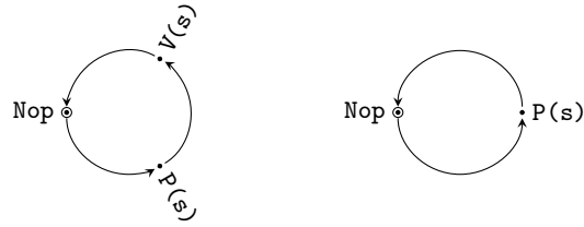
Figure 3: Conservative loop vs nonconservative loop.
