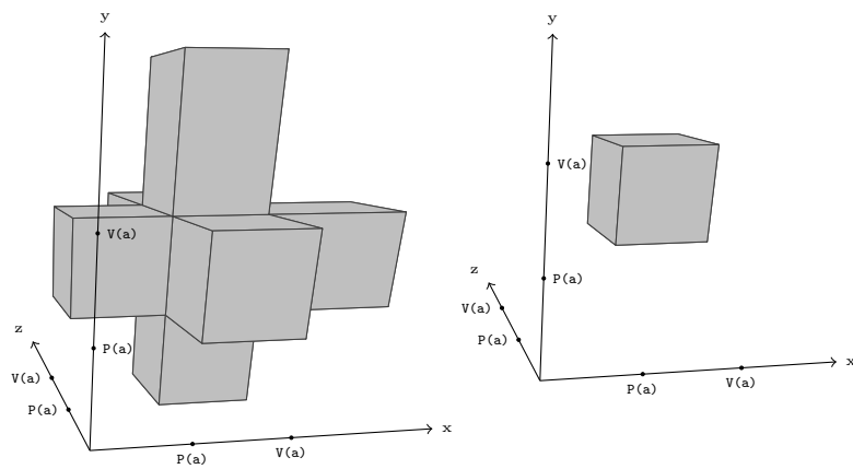
Figure 11: The tetrahemihexacron a.k.a. 3D Swiss Cross, and the 'floating' cube.
