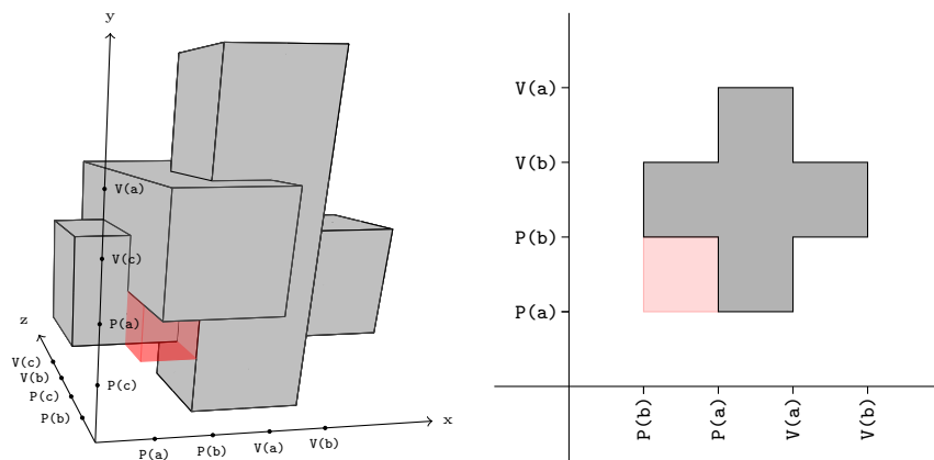
Figure 10: The three dining philosophers and the Swiss Cross with their deadlock attractors (in red).
