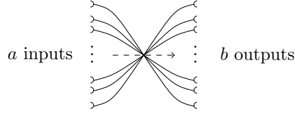
Figure 7: Ordered open stars.
