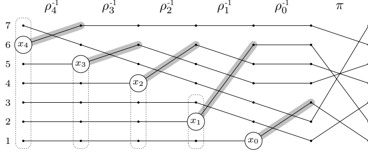
Figure 2: The rolling decomposition of the permutation \pi = (1\ 3)(2\ 7\ 6)(4\ 5) .
