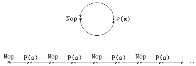
Figure 5: A nonconservative loop and its unfolding.
