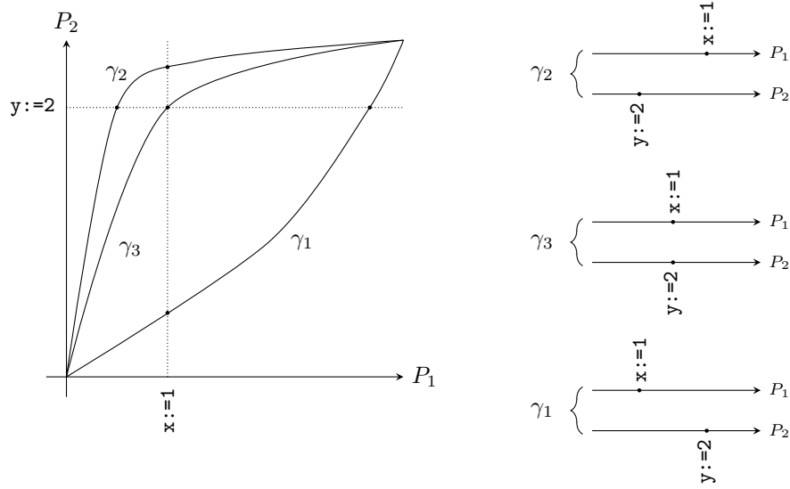
Figure 15: Timelines and sequences of multi-instructions interpreting weakly dihomotopic directed paths.
