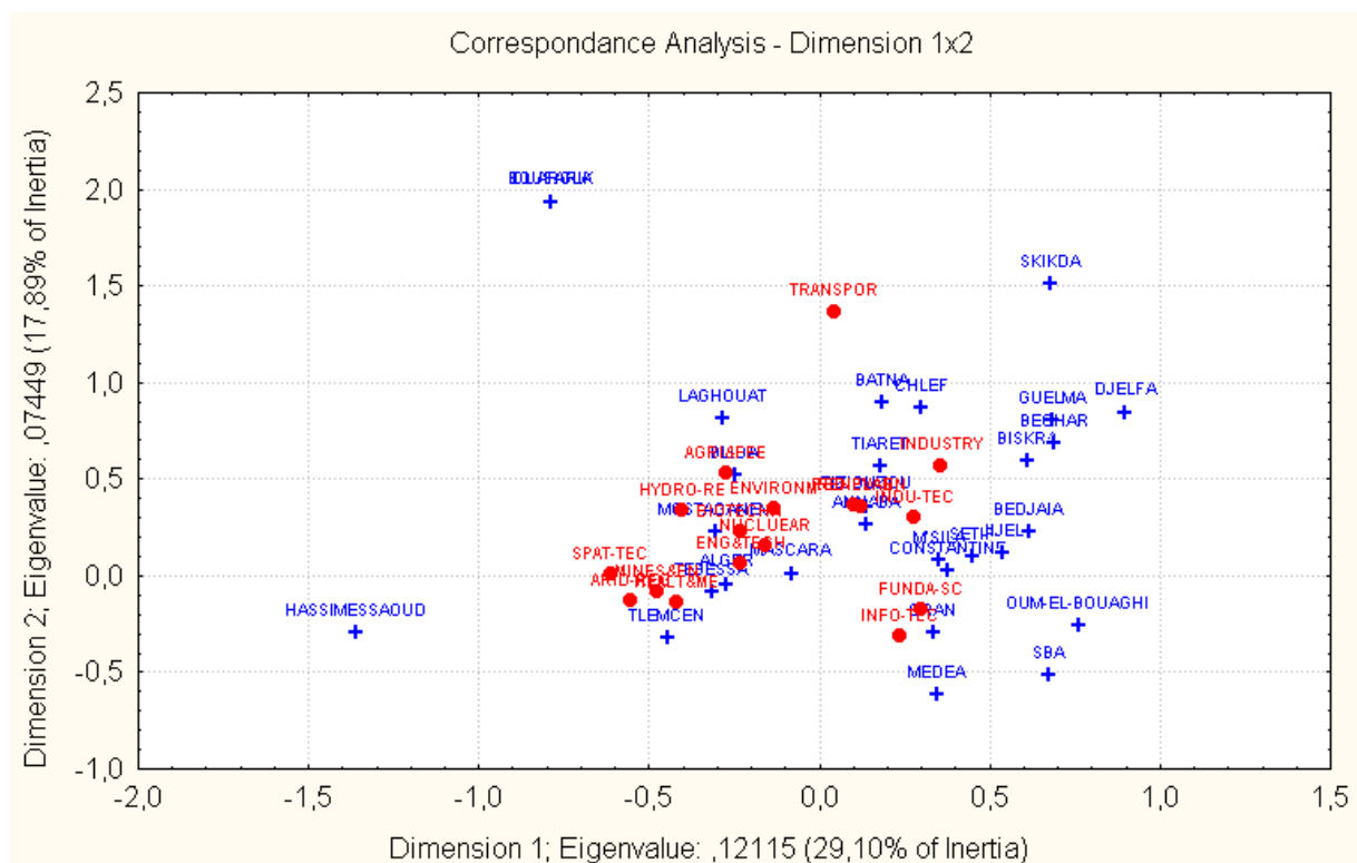
Figure 6: Map obtained with correspondence analysis of the matrix that was represented in Fig 5
