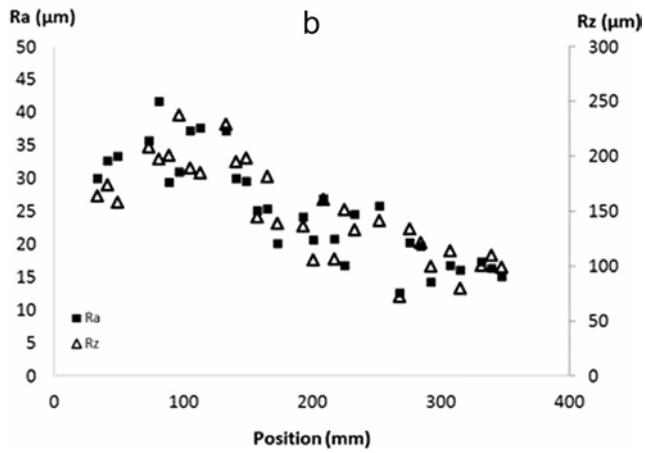
Fig. 4 Roughness profiles of ZE41 cast bar at a 6 and b 15 \cdot 10^{-4} MPa s^{-1} along cast bar length
