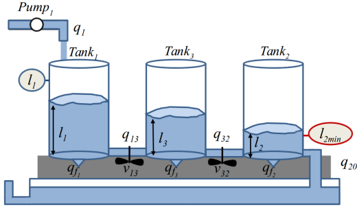
Figure 3. Water tank system.
