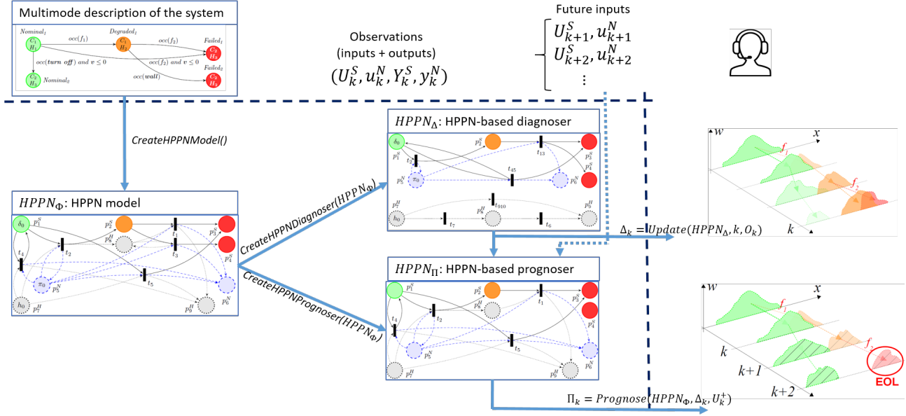
Figure 2. Overview of the health monitoring method.
