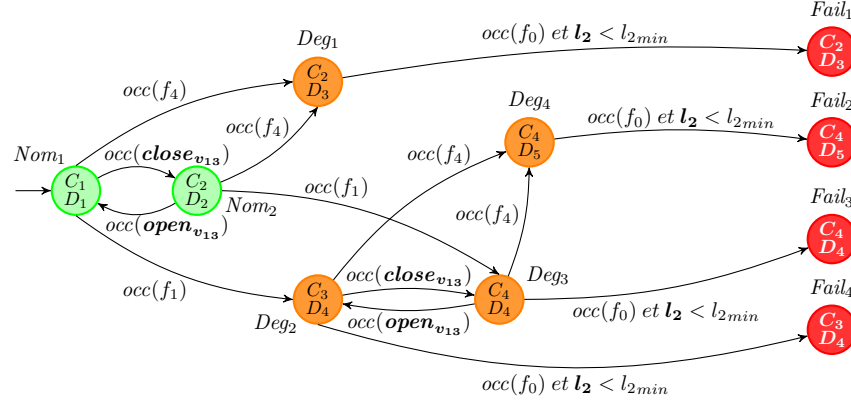
Figure 4. Multimode description of the health evolution of the water tank system.
