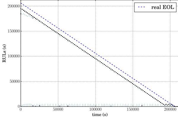
Figure 5. Scenario 1: RUL estimations.
