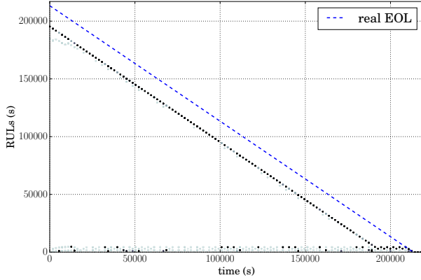
Figure 9. Scenario 3: RUL estimations.
