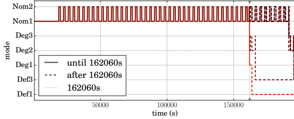
Figure 6. Scenario 1: Belief distribution on past and future trajectories of the system.
