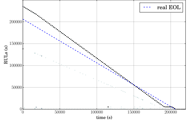
Figure 7. Scenario 2: RUL estimations.
