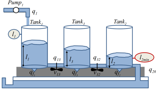
Figure 3. Water tank system.
