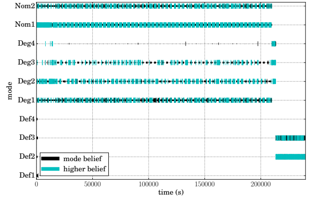
Figure 8. Scenario 3: Belief distribution on the system mode.
