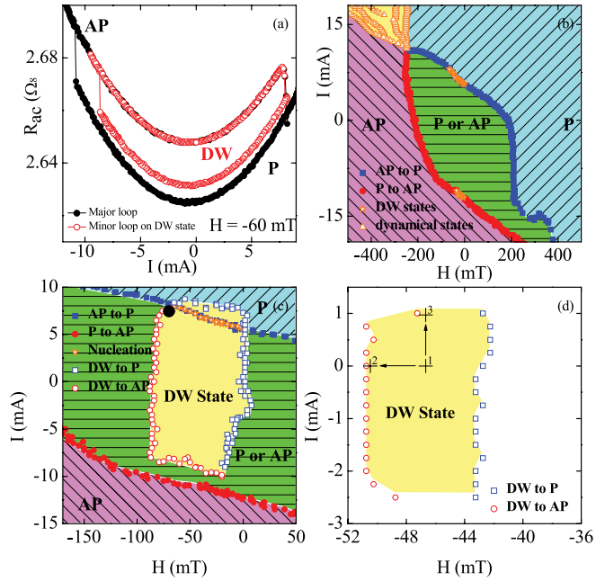
FIG. 1. (Color online) (a) Resistance of a 200 \times 100 \text{ nm}^2 hexagonal nanopillar spin-valve as a function of the injected current. The solids circles are for a major hysteresis loop. The opened red circles are for a minor hysteresis loop between the P state and a DW state formed by a single DW pinned in the free layer. (b) Experimental state diagram (magnetic field H vs injected current I ) obtained from major hysteresis loops such as the one of (a). Four regions are visible: One for the P state, one for the AP state, a bistability region, and a region where dynamical state are expected. (c) On top of the previous state diagram, the experimental state diagram of the DW state formed by a single DW pinned in the free layer obtained from minor hysteresis loops (a). The black circle indicates the region corresponding to the measurements of the telegraph noise signals on a similar sample and presented in Fig. 2. (d) Calculated state diagram of a DW state formed by a single pinned DW in the free layer (micromagnetic simulation).
