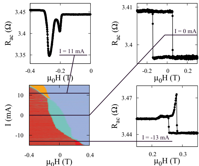
FIG. 4. (Color online) State diagram of an elliptical nanopillar spin valve of 50 nm by 300 nm with a hard layer made of [Co/Pt]/[Co/Ni] and a free layer made of [Co/Ni] obtained from the half sum method along with three characteristic hysteresis loops at I = -13 mA, I = 0 mA, and I = 11 mA.
