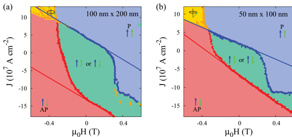
FIG. 10. (Color online) Experimental state diagrams of a hexagonal nanopillar spin valve with a hard layer made of [Co/Pt]/[Co/Ni] and a free layer made of [Co/Ni] of (a) 100 nm by 200 nm and of (b) 50 nm by 100 nm. The blue and red lines present what could correspond to the expected evolution of the switching current as a function of the applied magnetic field of our simple modeling.
