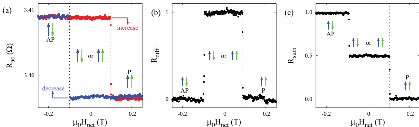
FIG. 2. (Color online) (a) ac-resistance variation as a function of the net applied magnetic field ( H_{\text{net}} ) under zero current for an elliptical nanopillar spin valve of 50 nm by 300 nm with a hard layer made of [Co/Pt]/[Co/Ni] and a free layer made of [Co/Ni] with a platinum layer on top. The net applied field is define as the applied field minus the average dipolar field coming from the hard layer ( H_{\text{net}} = H - H_{\text{dip}} ). The red and blue curves correspond to the field increasing and decreasing branches of the hysteresis loop. (b) Corresponding difference of the normalized resistances between the field increasing and decreasing branches of the hysteresis loop. (c) Corresponding half sum of the normalized resistances between the field increasing and decreasing branches of the hysteresis loop. The normalized resistances (R - R_P)/(R_{\text{AP}} - R_P) are plotted to remove the Joule heating contribution for the R_{\text{sum}} curve. These curves highlight three regions of different available magnetic configurations: the parallel (P) or the antiparallel (AP) states only or the bistable region.
