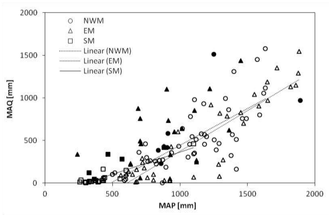
Fig. 2 Relationship between the Mean Annual Runoff (MAQ) and the Mean Annual Precipitation (MAP) for the three studied sub-regions (NWM, EM and SM). Plain symbols indicate karstic catchments in each sub-region.
