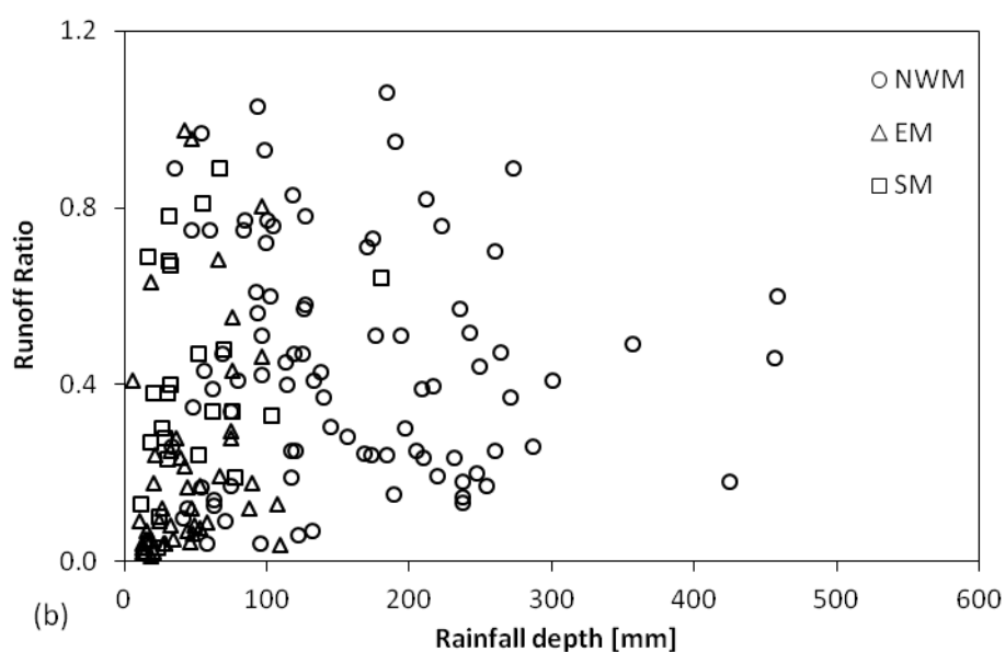
Fig. 7 Relationship between runoff depth and rainfall depth (a), and between runoff ratio and rainfall depth (b).
