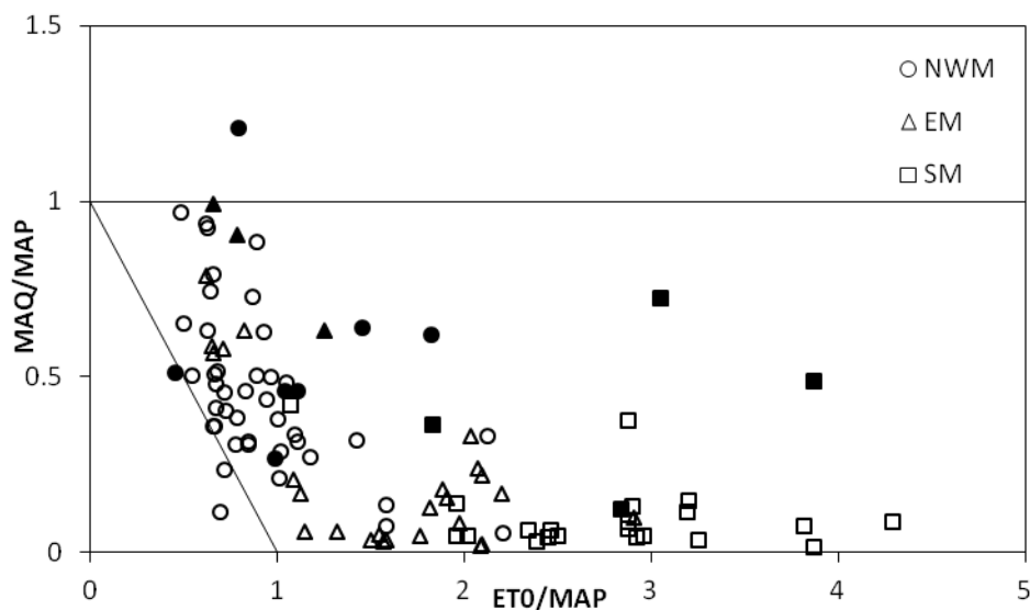
Fig. 2 Relationship between the Mean Annual Runoff (MAQ) and the Mean Annual Precipitation (MAP) for the three studied sub-regions (NWM, EM and SM). Plain symbols indicate karstic catchments in each sub-region.
