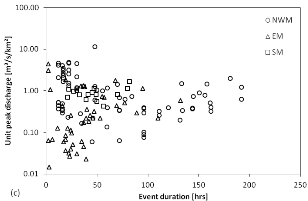
Fig. 6 Relationship between unit peak discharge and (a) catchment area, (b) rainfall depth and (c) event duration.
