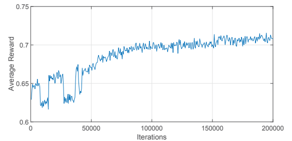
Fig. 6: Average perceived reward in the learning phase
