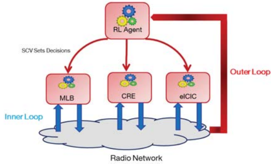
Fig. 3: PBSM based on RL
