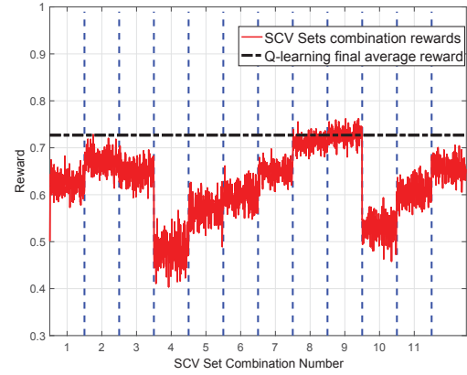
Fig. 5: SCV sets combination exhaustive search
