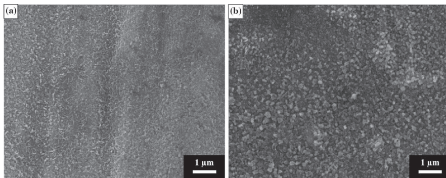
Fig. 5 SEM images (SE mode) of the surface of the oxide scale formed on the Ti6242S alloy a in synthetic air and b in 20%O 2 -80%Ar after 100 h at 650^\circ\text{C}
