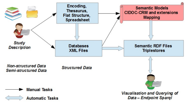
Figure 2. Architecture of ModRef project.
