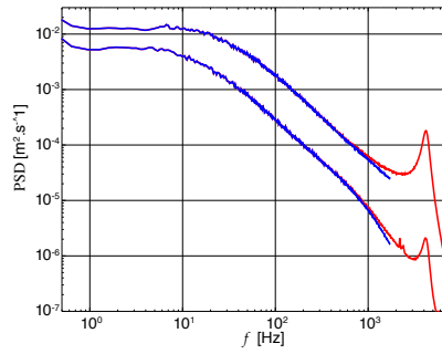
Fig. 7 Spectrum of velocity recorded with the miniature Pitot tube #1 for mean velocities 20 m/s and 45 m/s. The red curves represent the spectrum of the raw signal, where the Helmholtz resonance of the tube at 4.2 kHz can be seen. The blue lines simply show the same signal after removal of the Lorentzian peak.
