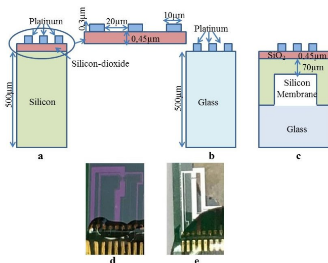
Figure 1: Schematic representation of- (a) silicon, (b) glass and (c) membrane based flow rate sensor; real fabricated sensor on (d) silicon and (e) glass substrate
