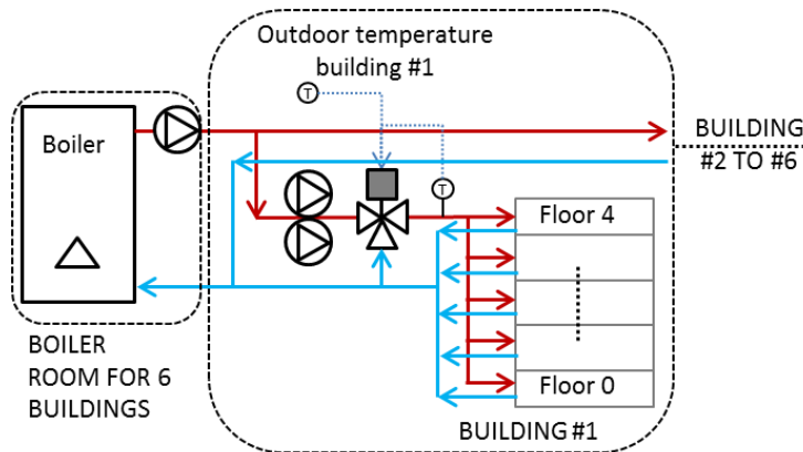
Figure 4 : Heating floor system regulation through substation – structure and heating curves
