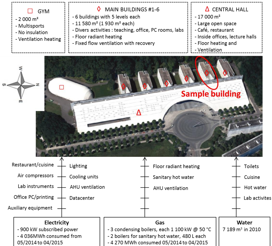
Figure 2. Details of the studied site – buildings, utilities and energy supplies. The red circle indicates the sample considered for instrumentation, measurements and building energy model validation presented in the following sections.
