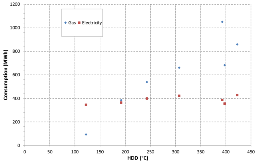
Figure 8. Monthly gas and electricity consumption as a function of the Heating Degree Days (HDD) during heating season from Oct-2014 to Apr-2015
