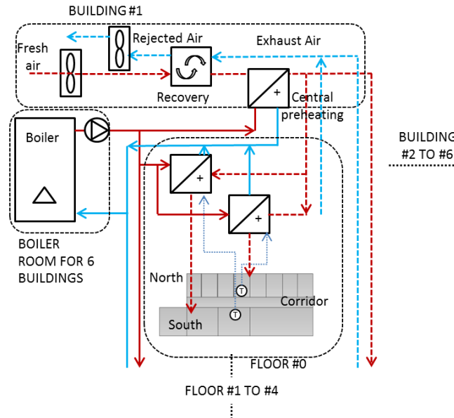
Figure 3. AHU and water systems provide indoor ventilation
