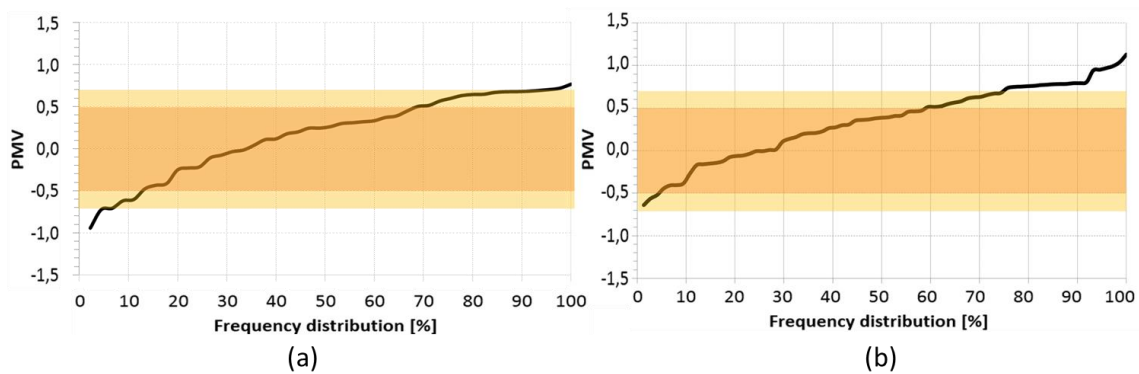
Figure 12. distribution of PMV for offices (a) and for classrooms (b). The darkest color represents, according to EN 15251, the comfort range of PMV for buildings belonging to category II; the brightest color the range for buildings in category III.
