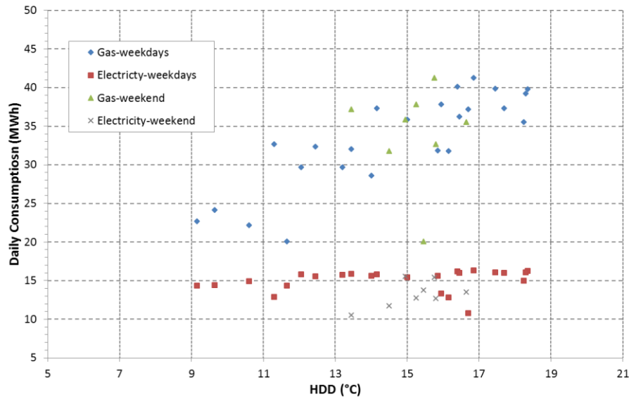
Figure 9. Gas and electricity consumption as a function of the Heating Degree Days (HDD) during heating season from Jan-13-2015 to Feb-13-2015
