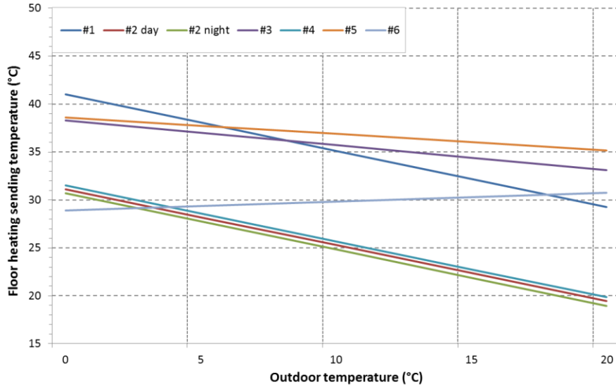
Figure 11. Heating curves of different substations. The substation heating floor equipment of building #2 and #4 where replaced in 2012 contrary to the four others.
