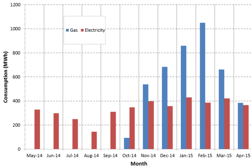
Figure 7 : Total energy consumption from May-2014 to Apr-2015
