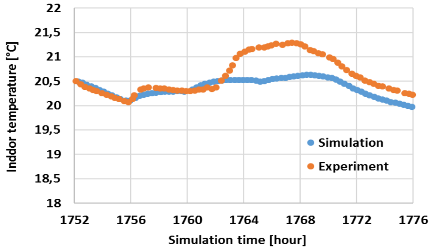
Figure 5 : Experimental and simulated indoor temperature variation during 24 hours
