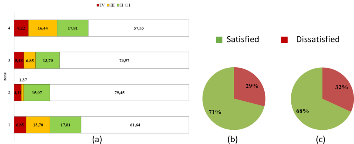
Figure 14. Percentage of time in comfort categories according to EN 15251 (a), percentage of comfort according to TSV (where the comfort range is [-1; 1]) (b); and TPV (where the comfort is [0]) (c).
