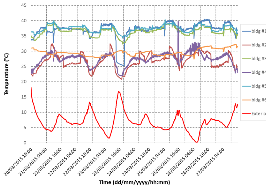
Figure 10. Comparison of identified heating curves between original and renovated substations
