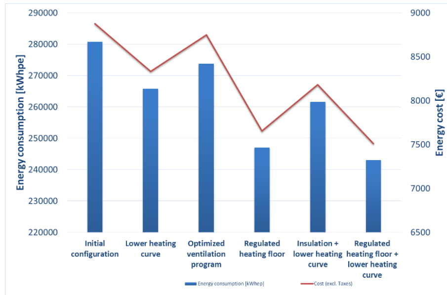
Figure 15. Thermal energy consumption and energy cost of the building #2 for different scenarios.
