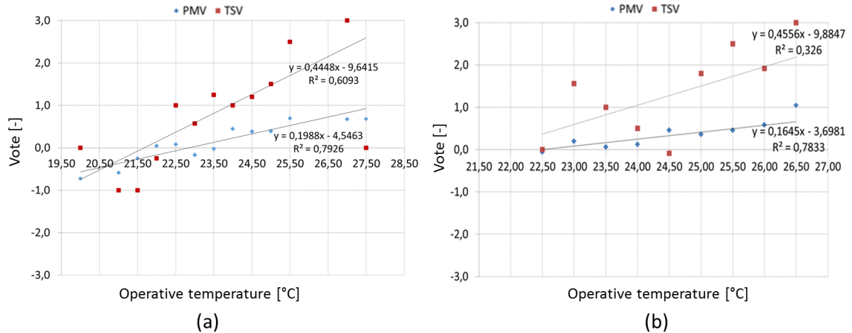
Figure 13. Correlation between T_{op} and PMV, T_{op} and TSV for offices (a) and classrooms (b)
