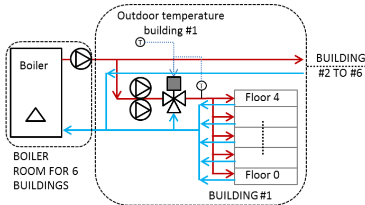
Figure 4 : Heating floor system regulation through substation – structure and heating curves
