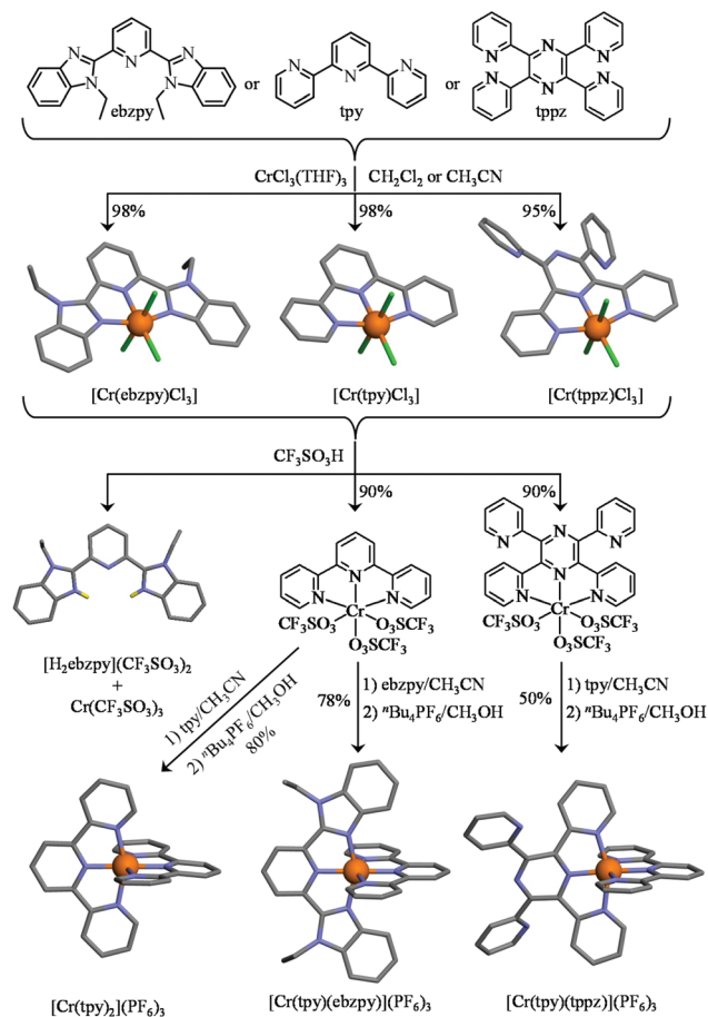
Fig. 4 Synthesis of the heteroleptic mononuclear chromium complexes. The molecular structures are those found in the crystal structures of [Cr(ebzipy)Cl 3 ].DMF ( 5 ), [Cr(tpy)Cl 3 ].(CH 3 ) 2 SO, 93 [Cr(tppz)Cl 3 ].2DMF ( 6 ), [Cr(tpy) 2 ](PF 6 ) 3 ·2.5CH 3 CN ( 2 ), [Cr(tpy)(ebzipy)](PF 6 ) 3 ·2CH 3 CN ( 7 ), [Cr(tpy)(tppz)](PF 6 ) 3 ·3CH 3 CN ( 8 ) and [H 2 (ebzipy)](CF 3 SO 3 ) 2 ( 10 ). The hydrogen atoms have been omitted for clarity. Color code: C = grey, N = blue, Cr = orange, Cl = green, H = yellow.
