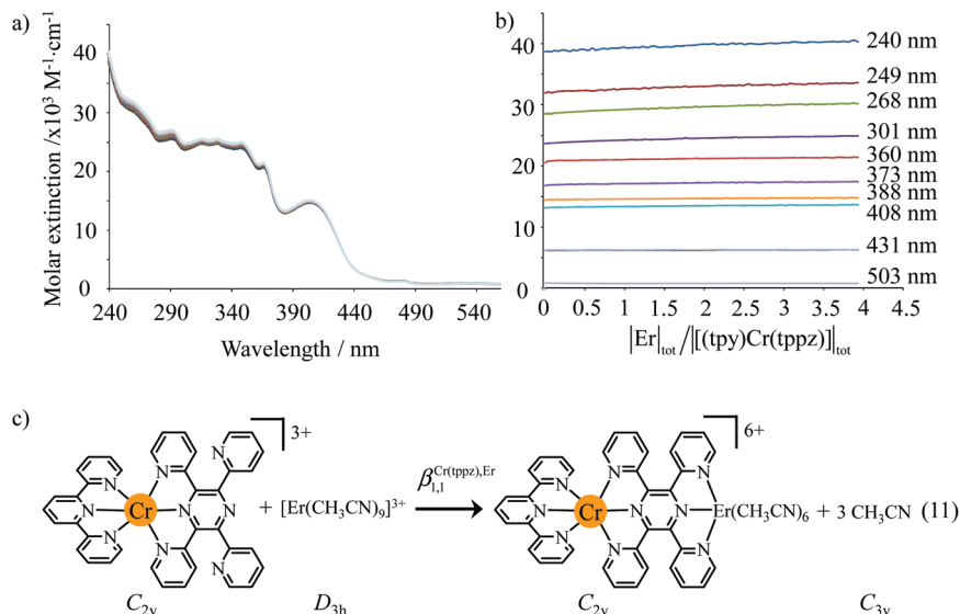
Fig. 10 (a) Variation of absorption spectra, (b) corresponding variation of molar extinctions and (c) proposed modeling ( \beta_{1,1}^{\text{Cr}(\text{tpz}),\text{Er}} \ll 50 ) for the titration of [(\text{tpy})\text{Cr}(\text{tppz})]^{3+} ( 2 \times 10^{-4} M) with \text{Er}(\text{CF}_3\text{SO}_3)_3 in acetonitrile (298 K).
