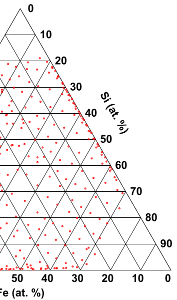
FIG. 6. Compositions in the Fe-Si-Ge thin film library as determined by high-throughput EDX measurements.
