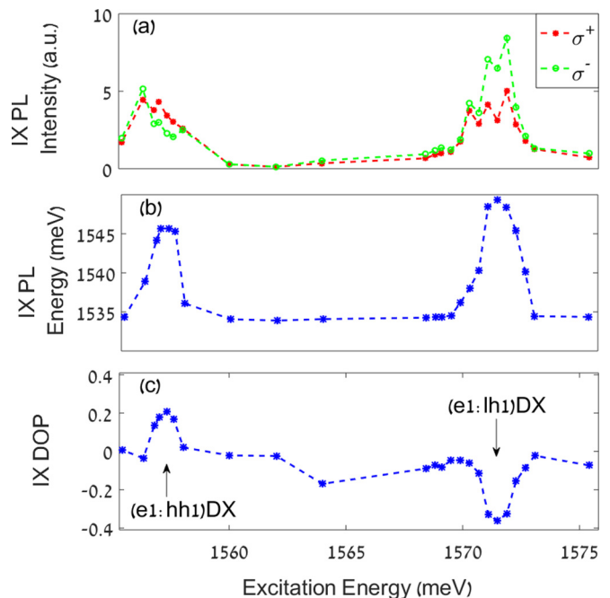
FIG. 6. Polarization-resolved PLE of IX. (a) The integrated PL intensity, monitored at the IX line for both polarizations. (b) The PL energy and (c) the degree of circular Polarization (DOP). A negative DOP means that the PL of the IX has the opposite circular polarization with respect to the circularly polarized exciting laser. The laser power here is 1.3 \mu W and is circularly polarized with \sigma^+ . The energies of (e1:hh1) DX and (e1:lh1) DX are pointed in (c) as a guide to the eye.
