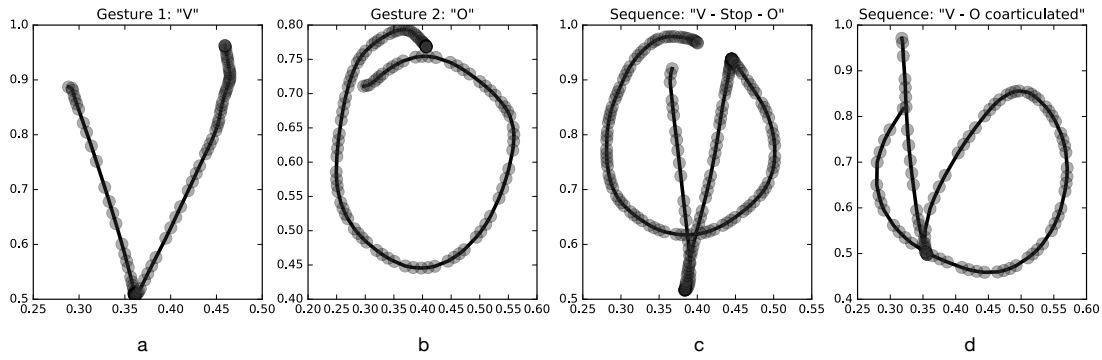
Figure 1: The gestures used in the experiment and several instances of their sequences. The two basic gestures are two-dimensional trajectories representing the symbols V (a) and O (b). Figures (c) and (d) respectively represent a sequence of gestures 1 and 2, either with a pause between, or rapidly without break.
