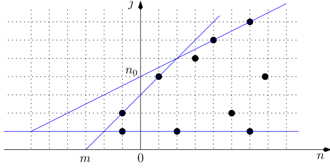
FIGURE 4. The support of the series A(y) , shown with dots, and the definition of m .
