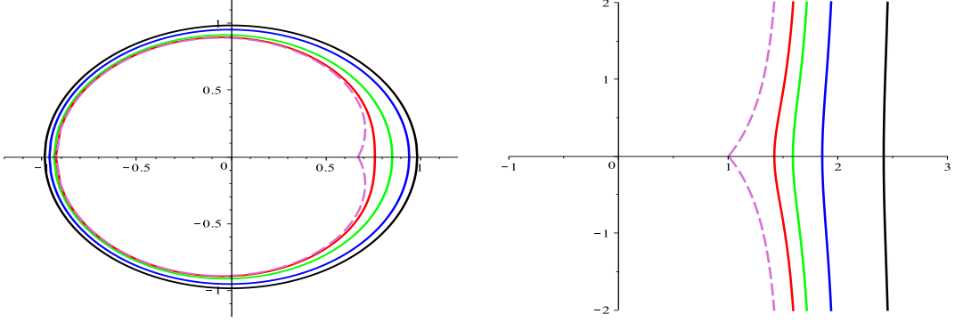
FIGURE 6. The curves \mathcal{L} for model #3 of Table 5 (for t = 0.03, 0.1, 0.2, 0.25 = 1/|\mathcal{S}| and 0.263185\dots as one moves closer to the origin) and for the reverse Kreweras model (second model in Table 4; from right to left, t = 0.2, 0.25, 0.28, 0.3 and 1/3 = 1/|\mathcal{S}| ). The dashed curve is obtained for a value t_c \geq 1/|\mathcal{S}| , where \mathcal{L} stops being smooth, but here we only consider values of t less than 1/|\mathcal{S}| .
