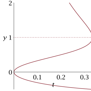
FIGURE 9. A plot of the three branches of K(y, y; t) = 0 against t for t \in [0, 1/3] .
