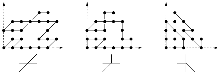
FIGURE 1. Three models of walks in the quadrant. The series Q(x, y; t) is algebraic for the first one, but only D-algebraic for the second. For the third one, it is not even D-algebraic.
