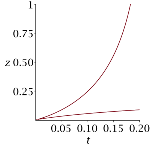
FIGURE 8. A plot of x_1(1+x_1) (bottom) and x_2(1+x_2) (top) for t \in [0, 1/5] in model #5.
