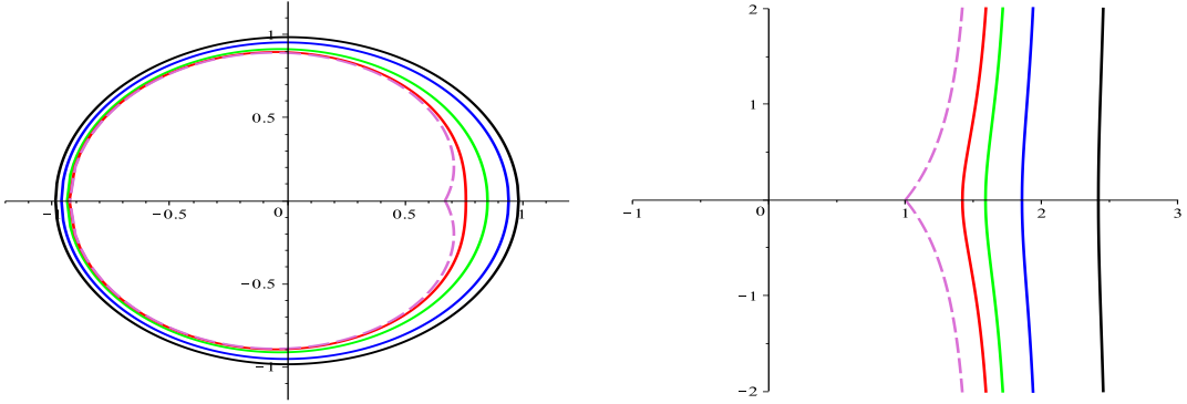
FIGURE 6. The curves \mathcal{L} for model #3 of Table 4 (for t = 0.03, 0.1, 0.2, 0.25 = 1/|\mathcal{S}| and 0.263185\dots as one moves closer to the origin) and for the reverse Kreweras model (second model in Table 3; t = 0.2, 0.25, 0.28, 0.3 and 1/3 = 1/|\mathcal{S}| from right to left). The dashed curve is obtained for a value t_c \geq 1/|\mathcal{S}| , where \mathcal{L} stops being smooth, but here we only consider values of t less than 1/|\mathcal{S}| .
