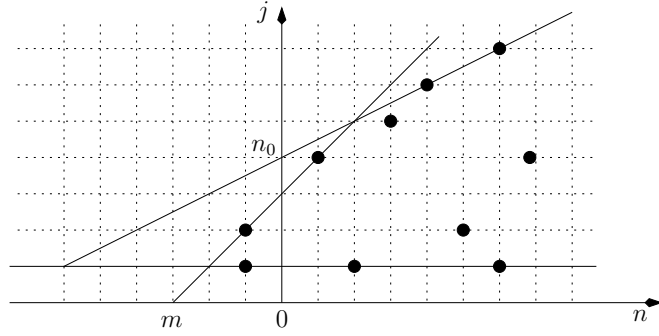
FIGURE 2. The support of the series A(y) , shown with dots, with the definition of m .
