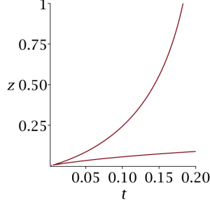
FIGURE 6. A plot of x_1(1+x_1) (bottom) and x_2(1+x_2) (top) for t \in [0, 1/5] in model #5.
