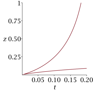
FIGURE 6. A plot of x_1(1+x_1) (bottom) and x_2(1+x_2) (top) for t \in [0, 1/5] in model #5.
