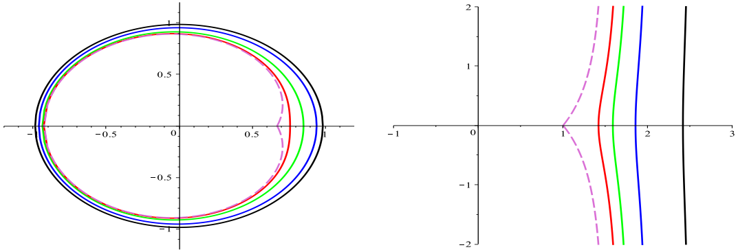
FIGURE 4. The curves \mathcal{L} for model #3 of Table 4 (for t = 0.03, 0.1, 0.2, 0.25 = 1/|\mathcal{S}| and 0.263185\dots as one moves closer to the origin) and for the reverse Kreweras model (second model in Table 3; t = 0.2, 0.25, 0.28, 0.3 and 1/3 = 1/|\mathcal{S}| from right to left). The dashed curve is obtained for a value t_c \geq 1/|\mathcal{S}| , where \mathcal{L} stops being smooth, but here we only consider values of t less than 1/|\mathcal{S}| .
