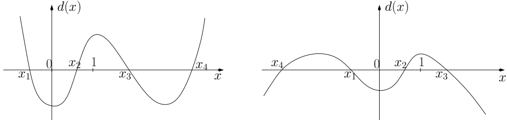
FIGURE 3. Plot of d(x) for x real: the main two possibilities, depending on the sign of x_4 . Note that x_1 may be non-negative, and x_4 may be +\infty .
