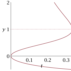
FIGURE 7. A plot of the three branches of K(y, y; t) = 0 against t for t \in [0, 1/3] .
