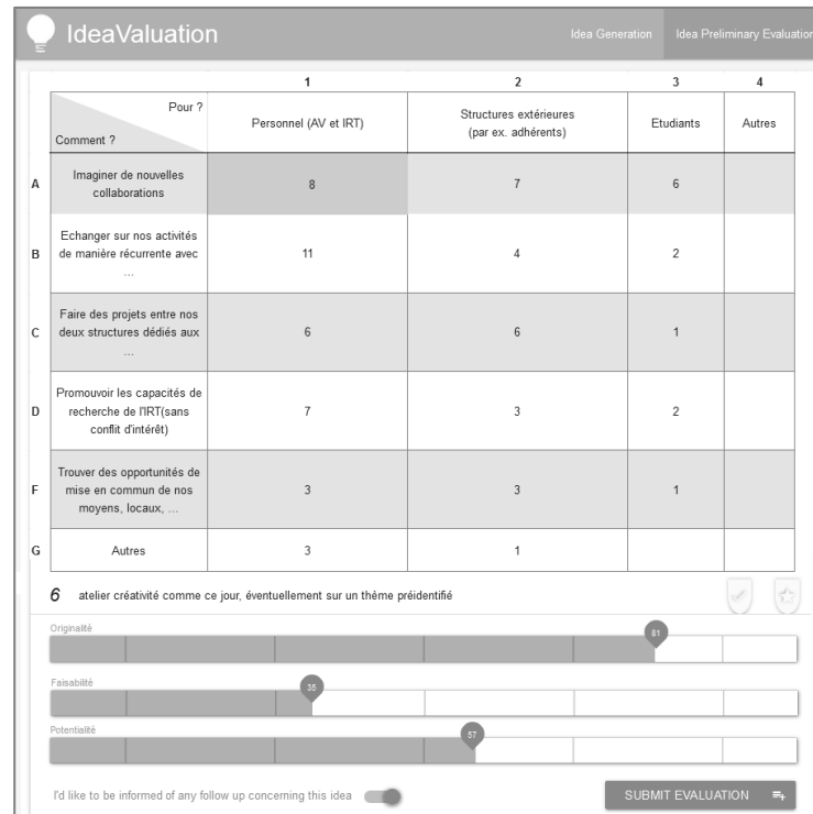
Figure 4. IdeaValuation's view into evaluation phase
