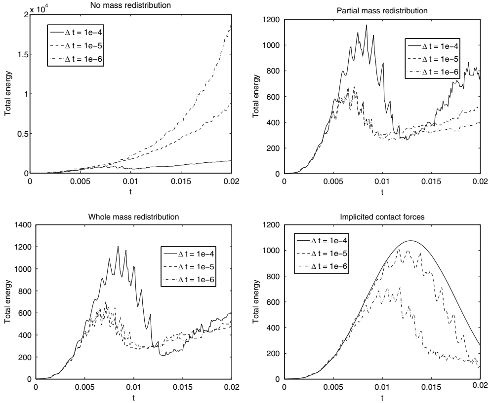
Fig. 7 Evolution of the energy for the following four situations: standard discretization, partial mass redistribution, whole-mass redistribution and standard discretization with implicated contact forces
