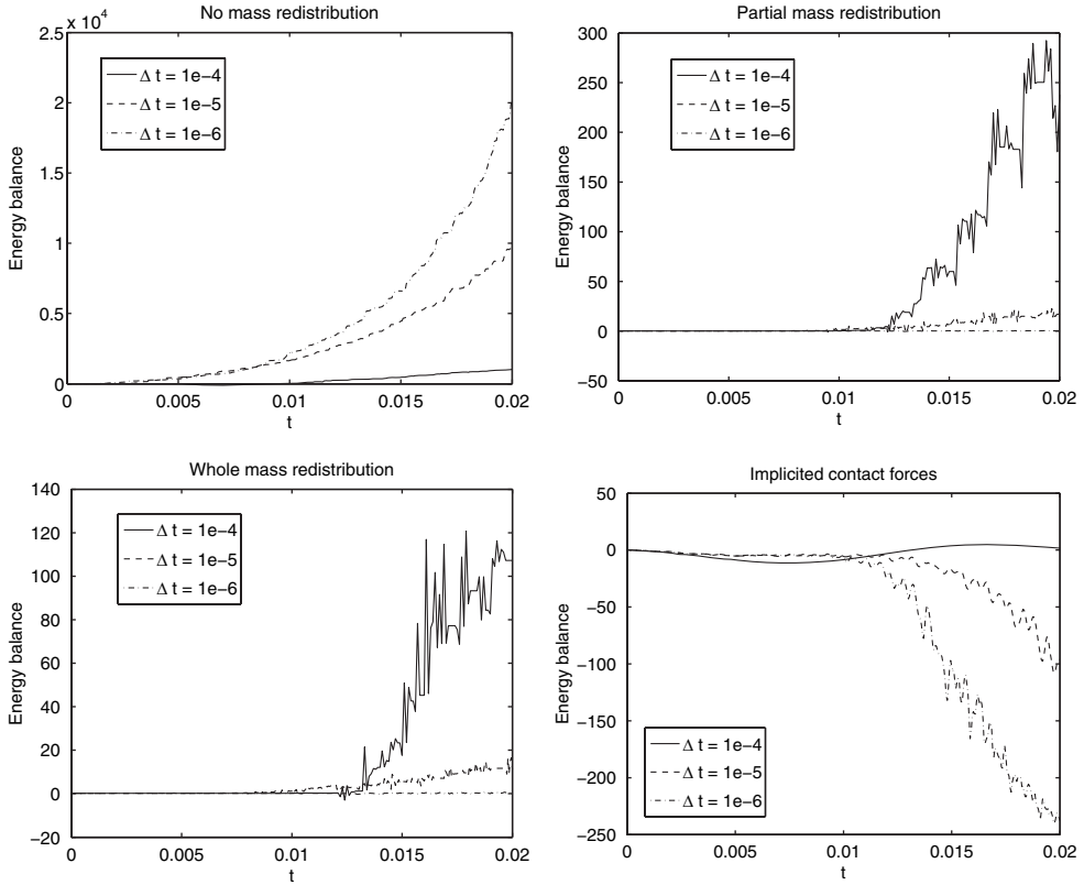
Fig. 8 Evolution of the difference between the total energy and the energy transferred by friction
