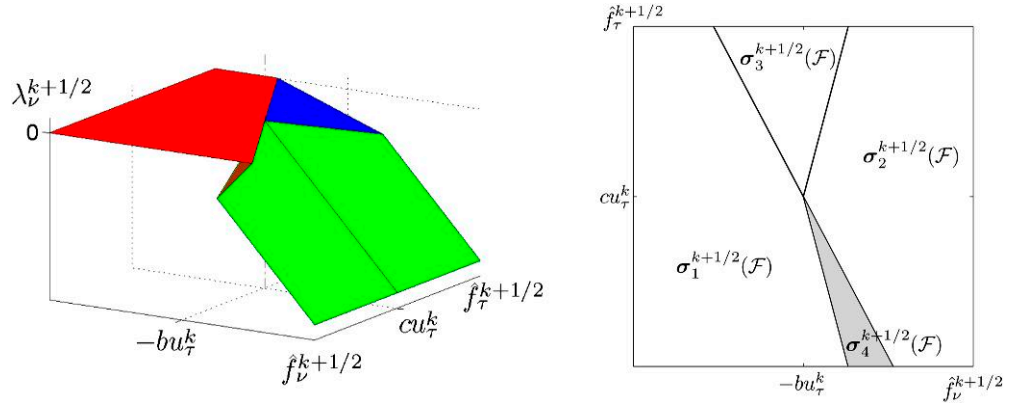
Fig. 4 Structure of the solution for \mathcal{F} \in (c/b, +\infty)
