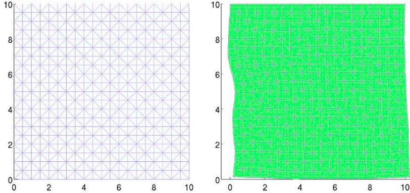
Fig. 6 Structured mesh of the square \{(x_1, x_2) \in ]0, 10 \text{ cm}[ \times ]0, 10 \text{ cm}[ and an example of deformation (at t = 0.01 \text{ s} ). The rigid foundation lies at x_2 = 0 and has a constant horizontal velocity of 20 \text{ m/s} . The structure is clamped on its top ( x_2 = 10 \text{ cm} )
