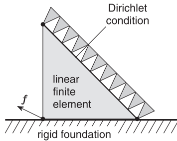
Fig. 2 Geometry of the elementary example
