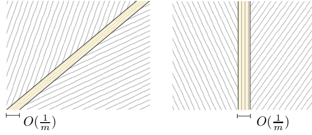
FIGURE 7. Buffer zones (yellow) in action.
