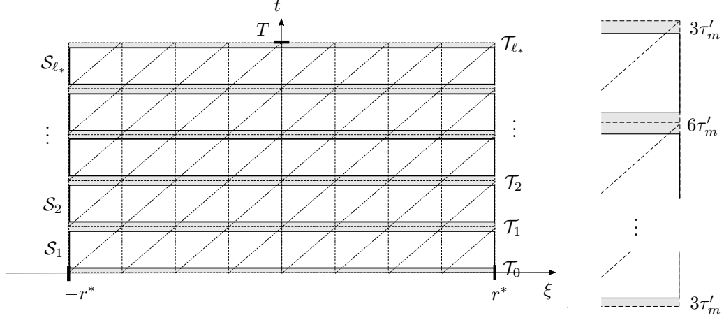
FIGURE 9. The Slabs \mathcal{S}_i (white boxes) and transition zones \mathcal{T}_i (gray)
