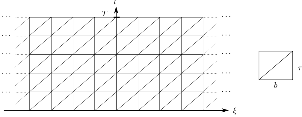
FIGURE 5. The triangulation \Sigma(\tau, b)
