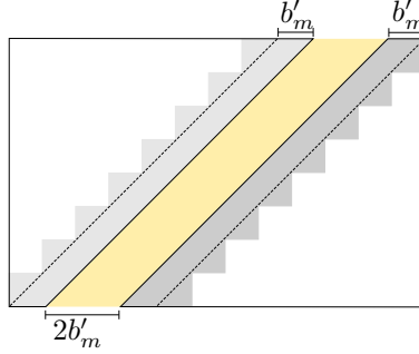
FIGURE 14. On each reduced triangle \triangle , the function \tilde{\Lambda}_{m,n} takes value \lambda_{\triangle} on the gray regions, no matter \lambda_{\triangle} \geq 1 or \lambda_{\triangle} < 1 . The gray regions stretch a distance b'_m from the buffer zone into the reduced triangles.
