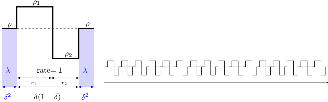
FIGURE 4. Expected macroscopic density under the intermittent construction. Here \rho_1 > \rho_2 \in [0, 1] are the unique solutions of the equation \rho_i(1 - \rho_i) = \kappa , and r_1, r_2 are such that r_1 + r_2 = \delta(1 - \delta) , r_1\rho_1 + r_2\rho_2 = (r_1 + r_2)\rho .
