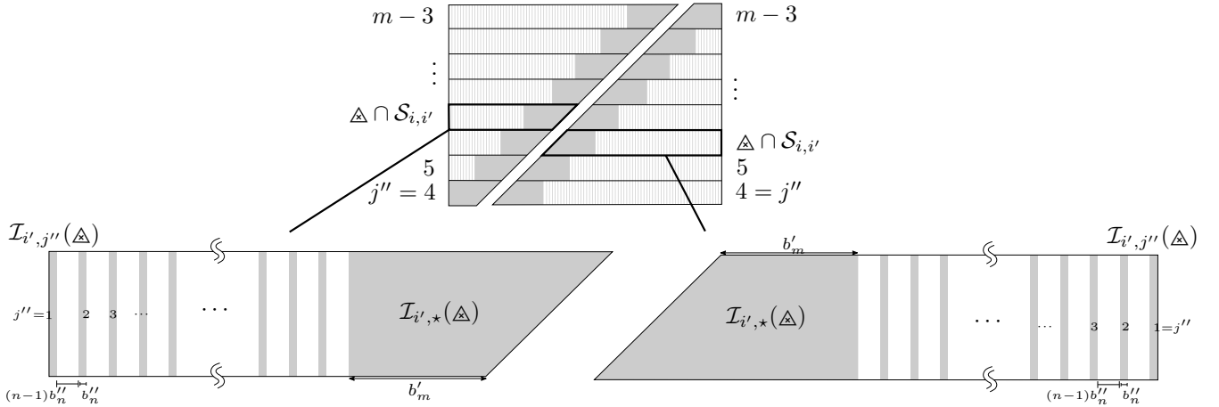
FIGURE 11. Intermittent zones (gray) on a given \underline{\Delta} with \lambda_{\underline{\Delta}} < 1
