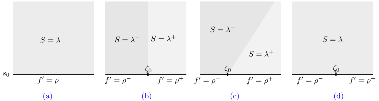
FIGURE 8. Four types of (S, f)
