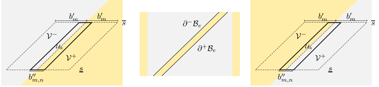
FIGURE 13. The regions \mathcal{U}_k , \mathcal{V}^+ and \mathcal{V}^-
