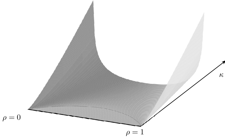
FIGURE 2. Graph of the rate density J(\kappa, \rho) . The dash line is where \kappa = \rho(1 - \rho) .
