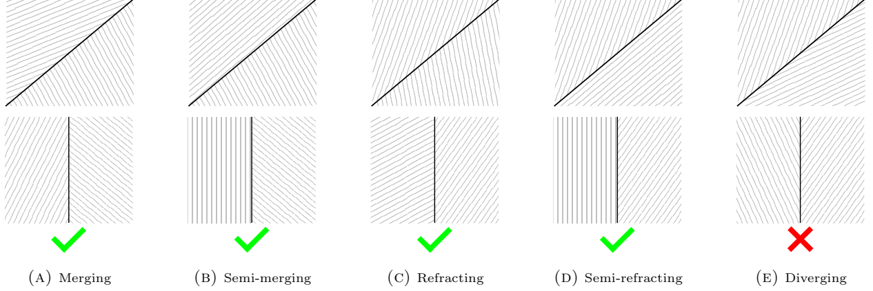
FIGURE 6. Configurations at a vertical or diagonal edge
