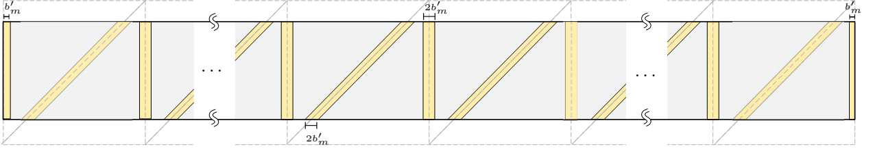
FIGURE 10. Buffer zones (yellow) and reduced triangles (gray)
