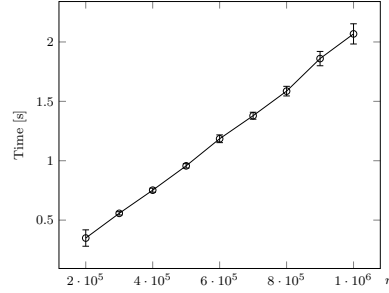
(b) Interpolation of average execution times of Table 17a.
