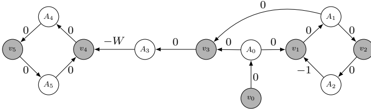
(b) The corresponding MPG G_{\mathcal{H}_W} computed by Algorithm 1.
