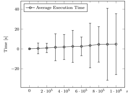
(b) Interpolation of average execution times of Test 1.
