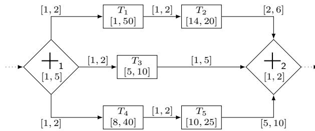
Fig. 1: A simple workflow schema excerpt with three parallel flows of execution.
