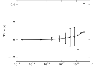
(b) Interpolation of average execution times in Table 21a.
