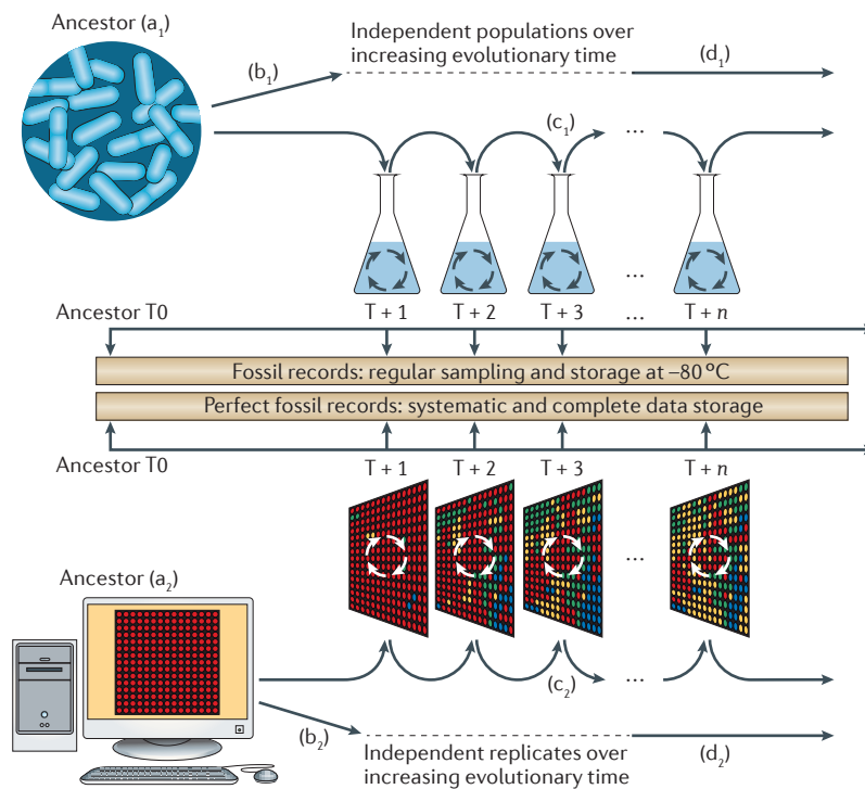
Figure 9 – Parallel in vivo (top) and in silico (bottom) experimental evolution. The experiments conducted in vivo are mimicked in the computational framework. Figure from (Hindr e et al. , 2012).
