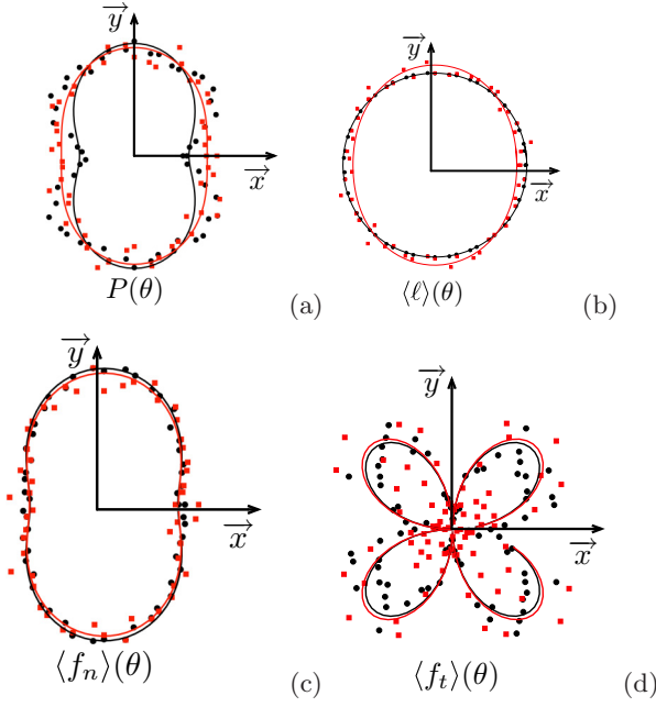
FIG. 11. Polar representation of the functions P(\theta) (a), \langle \ell \rangle(\theta) (b), \langle f_n \rangle(\theta) (c), and \langle f_t \rangle(\theta) (d), for (s,b) = (0.2,1) (black circles) and (s,b) = (0.9,1) (red squares). The corresponding harmonic approximations are drawn as solid lines.
