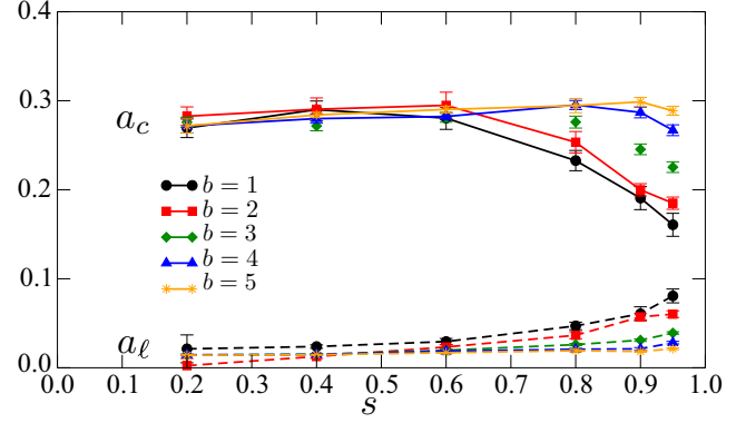
FIG. 12. Contact orientation a_c (line) and branch length a_\ell (dashed line) anisotropies as functions of s for all values of b . Error bars represent the standard deviation in the steady state.
