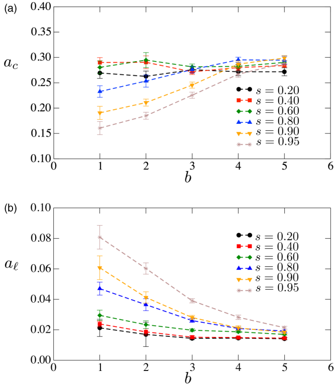
FIG. 13. Contact anisotropies a_c (a) and branch length anisotropies a_l (b) as functions of b for all values of s . Error bars represent the standard deviation in the steady state.
