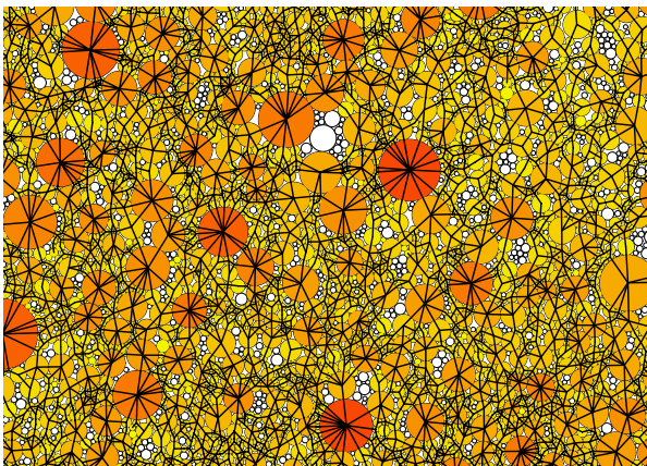
FIG. 7. Contact network (black lines) and particle connectivity (color scale) for (s,b) = (0.9,1) (a) and (s,b) = (0.9,5) (b). Color intensity is proportional to the grains' number of contacts. The floating particles (i.e., particles with zero or one contact) are shown in white.
