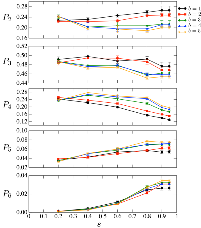
FIG. 9. Particle connectivity, defined as the proportion P_c of particles with exactly c contacts, as a function of s for all values of b . The error bars represent the standard deviation in the steady state.
