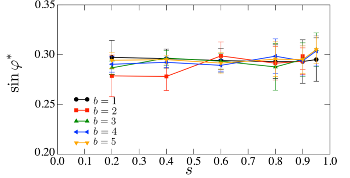
FIG. 5. Sine of the internal friction angle in the steady state \sin \varphi^* as a function of s for all values of b . Error bars represent the standard deviation in the steady state.
