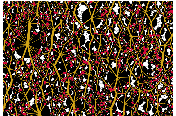
FIG. 10. Snapshots of the force network for (a) (s, b) = (0.2, 2) and (b) (s, b) = (0.9, 5) . Floating particles are shown in white and normal forces are represented by the thickness of the segments joining the particle centers. The red circles in the contact points represent friction mobilization, their diameter being proportional to the friction mobilization index (see text for definition).
