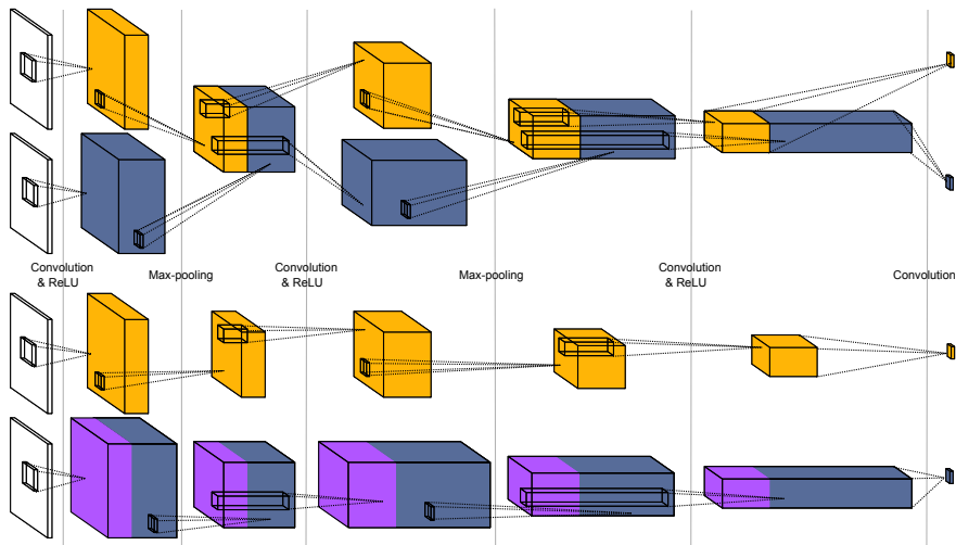
Figure 1: Feature map sharing. Top : Two-stage OnionNet. Bottom : A corresponding non-sharing cascade. In OnionNet, the first stage (S1, orange) shares its intermediate feature maps (visualized as cubes) with the second stage (S2, blue). Without sharing the stages are independent and S2 has to be evaluated fully, recomputing certain features (purple).
