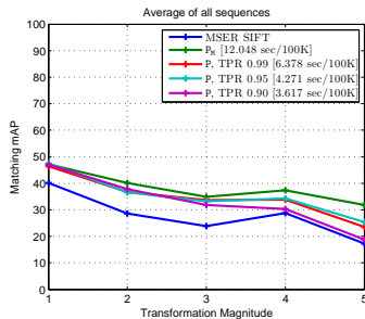
Figure 2: Descriptor matching (LDB).
