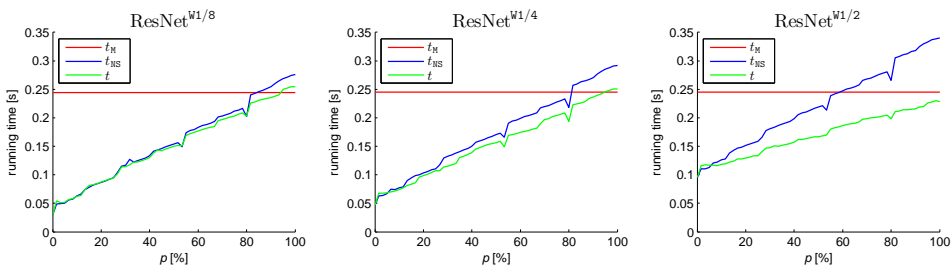
Figure 4: Empirical running times for cascades based on ImageNet ResNet-34 B network [L6] created by allocating 1/8 , 1/4 , or 1/2 of feature channels in each convolutional layer to S1 and leaving the rest in S2; both stages are of the same depth. The notation is identical to Figure 3 and the conclusions from Section 5.2 hold here as well.
