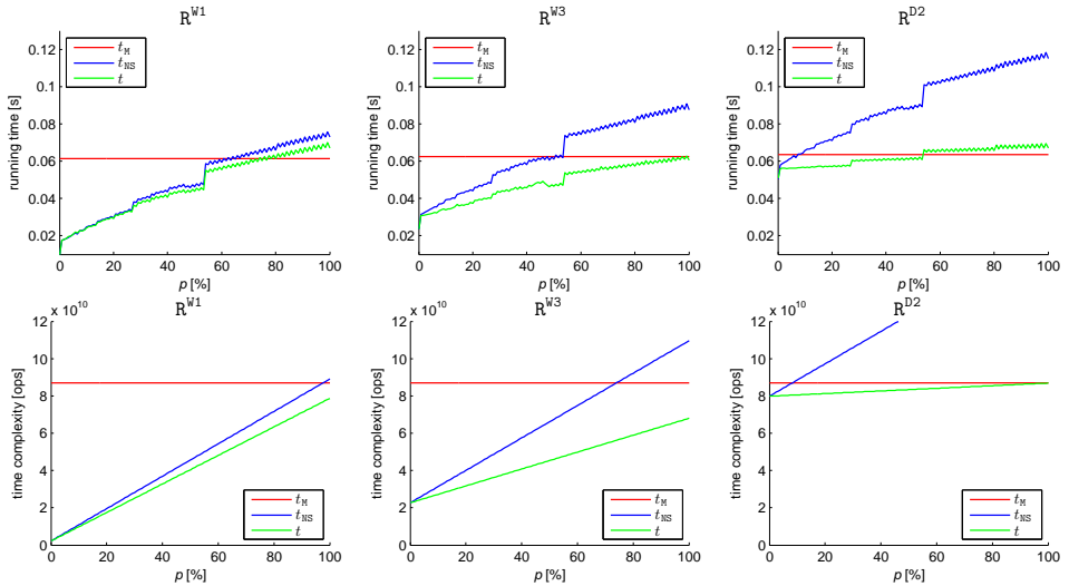
Figure 3: Empirical running times (first row) and time complexities (second row) for R_M -based cascades as functions of the percentage p of examples passing S1. Sharing cascade ( t ) is compared with a corresponding non-sharing baseline ( t_{NS} ) and its monolithic baseline ( t_M ).
