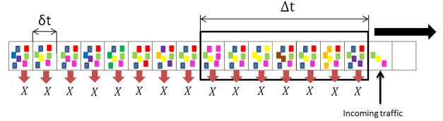
Figure 2. Feature space computation at the end of each micro-time-slot of \delta t seconds
