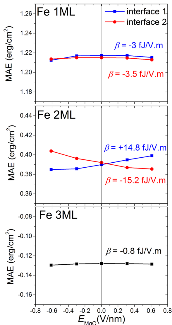
FIG. 5. On-site projected MAE as a function of E_{\text{MgO}} calculated for the first, second, and third Fe monolayers. The slope \beta of the MAE variation is evaluated and displayed for each ML.
