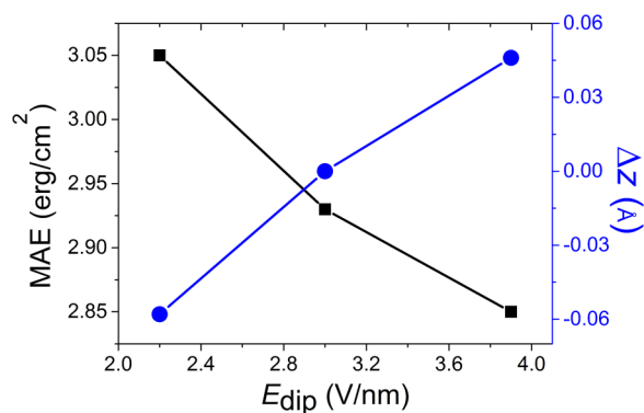
FIG. 4. The variation of the total MAE of the supercell, comprising two interfaces, as a function of the interfacial electric dipole E_{dip} which is modulated by the shift of the Mg position with respect to the O plane \Delta Z .
