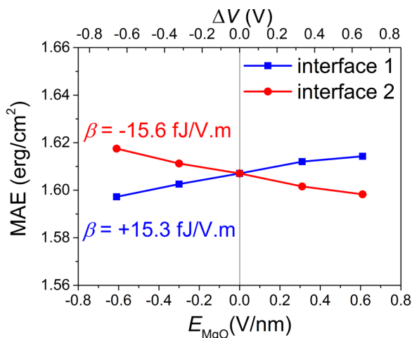
FIG. 3. The variation of the total magnetic anisotropy energy (MAE) per interface, comprising the first and second Fe monolayers, as a function of the electric field in the bulk of MgO ( E_{MgO} ) calculated by applying an electric field ranging from -2 to 2 V/nm in the vacuum region of the MgO/Fe/MgO supercell. The data points are linearly fitted to evaluate the slope \beta associated with the PMA response to the electric field.
