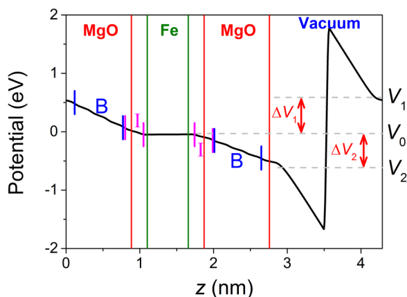
FIG. 1. Induced changes in the electrostatic potential under an electric field of -2 \text{ V/nm} applied in the vacuum region of a MgO/Fe/MgO supercell. The vertical red and green lines represent the boundaries between MgO and Fe layers, respectively. Two different regions of the potential gradient are identified in the bulk of MgO and at the Fe interface, designated by B and I, respectively. \Delta V_1 and \Delta V_2 designate the potential difference across the MgO where the reference potential V_0 is set as the Fe potential.
