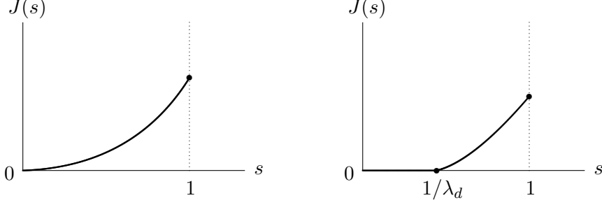
FIGURE 6. Qualitative plots of s \mapsto J(s) for d = 2 and d \geq 3 .
