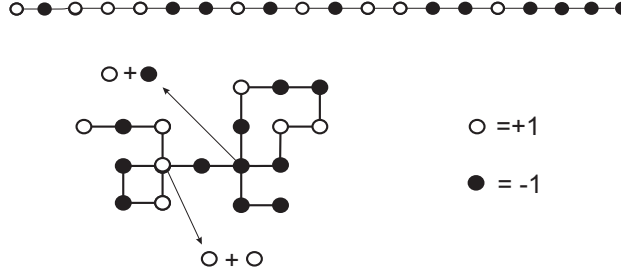
FIGURE 1. Top: A polymer chain of length n = 20 carrying (\pm 1) -valued random charges. Bottom: The charges only interact at self-intersections: in the picture monomers i = 4 , j = 8 meet and repel each other, while monomers i = 10 , j = 18 meet and attract each other.
