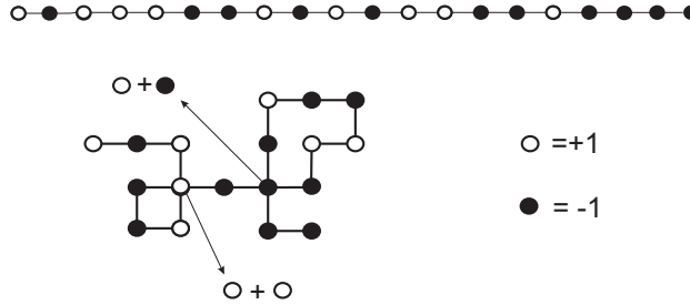
FIGURE 1. Top: A polymer chain of length n = 20 carrying (\pm 1) -valued random charges. Bottom: The charges only interact at self-intersections: in the picture monomers i = 4 , j = 8 meet and repel each other, while monomers i = 10 , j = 18 meet and attract each other.
