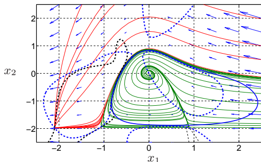
Fig. 2. The dashed light blue lines depict the set of points satisfying \dot{R}(x) = \langle \nabla R(x), f(x) \rangle = 0 , the dashed black lines depict the set \dot{V}(x) = \langle \nabla V(x), f(x) \rangle = 0 . The boundary of the RA lies in the set where \dot{R}(x) is negative.
