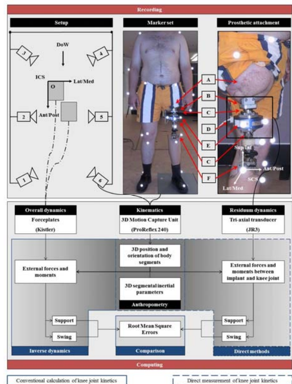
Fig. 1. Overview of conventional calculation and direct measurement of knee joint forces and moments for individuals with transfemoral amputation highlighting the computing with inverse dynamics and direct methods as well as the recording of input data including the setup of motion analysis laboratory, marker set and prosthetic attachment featuring the residuum (A), osseointegrated implant (B), pyramidal adaptors (C), serial cable (D), transducer (E), and knee joint (F). DoW: Direction of Walking, ICS: Inertial Coordinate System, SCS: thigh Segment Coordinate System, Lat/Med: lateral/medial axis, Ant/Post: anterior/posterior axis, Sup/Inf: superior/inferior axis.
