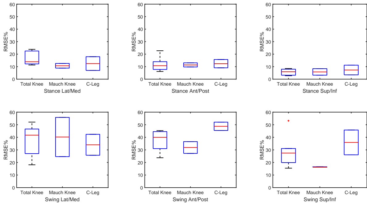
Fig. S1. Box-and-Whisker plots (i.e., median, lower and upper quartiles, minimum and maximum, and outlier “+”) of RMSE% for the lateral/medial (Lat/Med), anterior/posterior (Ant/Post), and superior/inferior (Sup/Inf) forces for the three hydraulic knees ( n = 6 for Total Knee, n = 2 for Mauch Knee, and n = 2 for C-Leg, the three gait trials of each participant collated together) during the stance and swing phases of gait.
