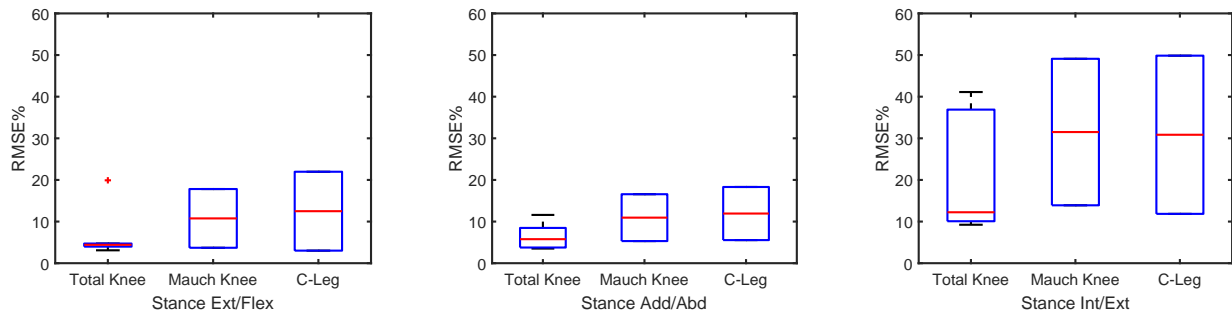
Fig. S2. Box-and-Whisker plots (i.e., median, lower and upper quartiles, minimum and maximum, and outlier “+”) of RMSE% for the extension/flexion (Ext/Flex) adduction/abduction (Add/Abd), and internal/external (Int/Ext) moments for the three hydraulic knees ( n = 6 for Total Knee, n = 2 for Mauch Knee, and n = 2 for C-Leg, the three gait trials of each participant collated together) during the stance phase of gait.
